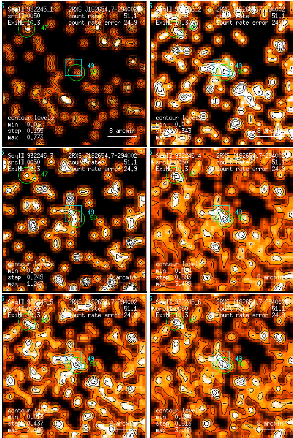
Figure 50: RASS 932245: detection 0050: band rate images, Gaussian filter: (1) PSPC channels 11 – 41, (2) 52 – 90, (3) 91 – 201, (4) 11 – 235, (5) 52 – 201, (6) 11 – 201. Broad band rates in counts/ks. Band rate contour levels in counts/ks/arcmin 2 .
