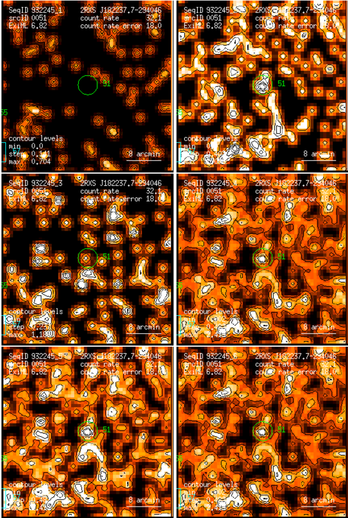
Figure 51: RASS 932245: detection 0051: band rate images, Gaussian filter: (1) PSPC channels 11 – 41, (2) 52 – 90, (3) 91 – 201, (4) 11 – 235, (5) 52 – 201, (6) 11 – 201. Broad band rates in counts/ks. Band rate contour levels in counts/ks/arcmin 2 .
