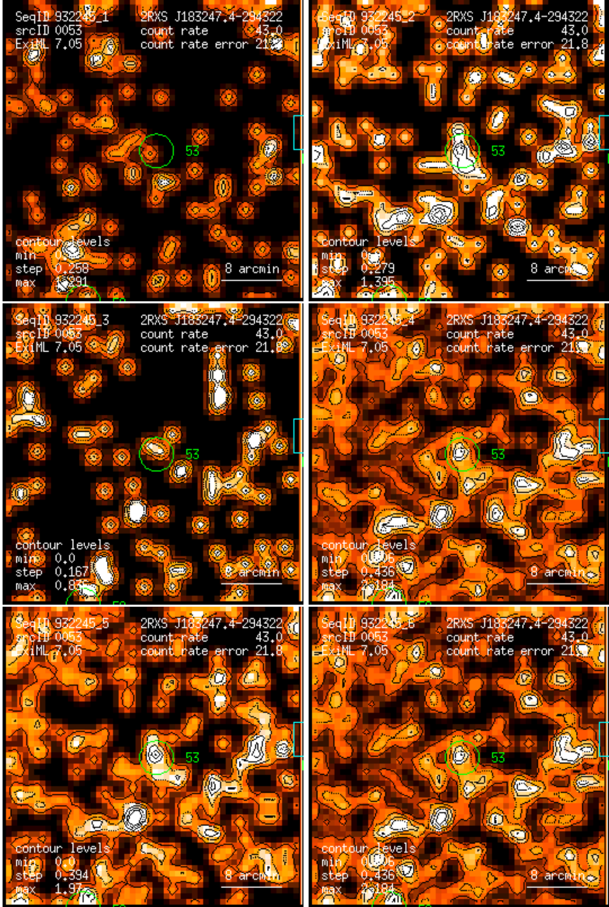
Figure 53: RASS 932245: detection 0053: band rate images, Gaussian filter: (1) PSPC channels 11 – 41, (2) 52 – 90, (3) 91 – 201, (4) 11 – 235, (5) 52 – 201, (6) 11 – 201. Broad band rates in counts/ks. Band rate contour levels in counts/ks/arcmin 2 .
