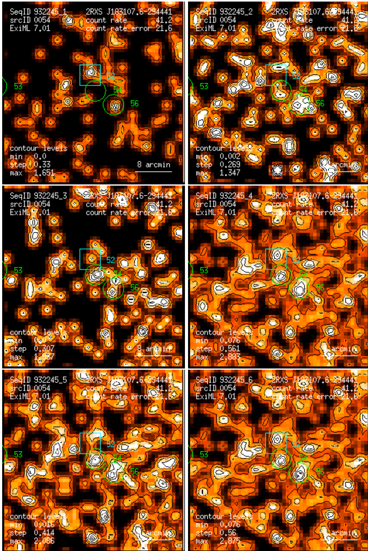
Figure 54: RASS 932245: detection 0054: band rate images, Gaussian filter: (1) PSPC channels 11 – 41, (2) 52 – 90, (3) 91 – 201, (4) 11 – 235, (5) 52 – 201, (6) 11 – 201. Broad band rates in counts/ks. Band rate contour levels in counts/ks/arcmin 2 .
