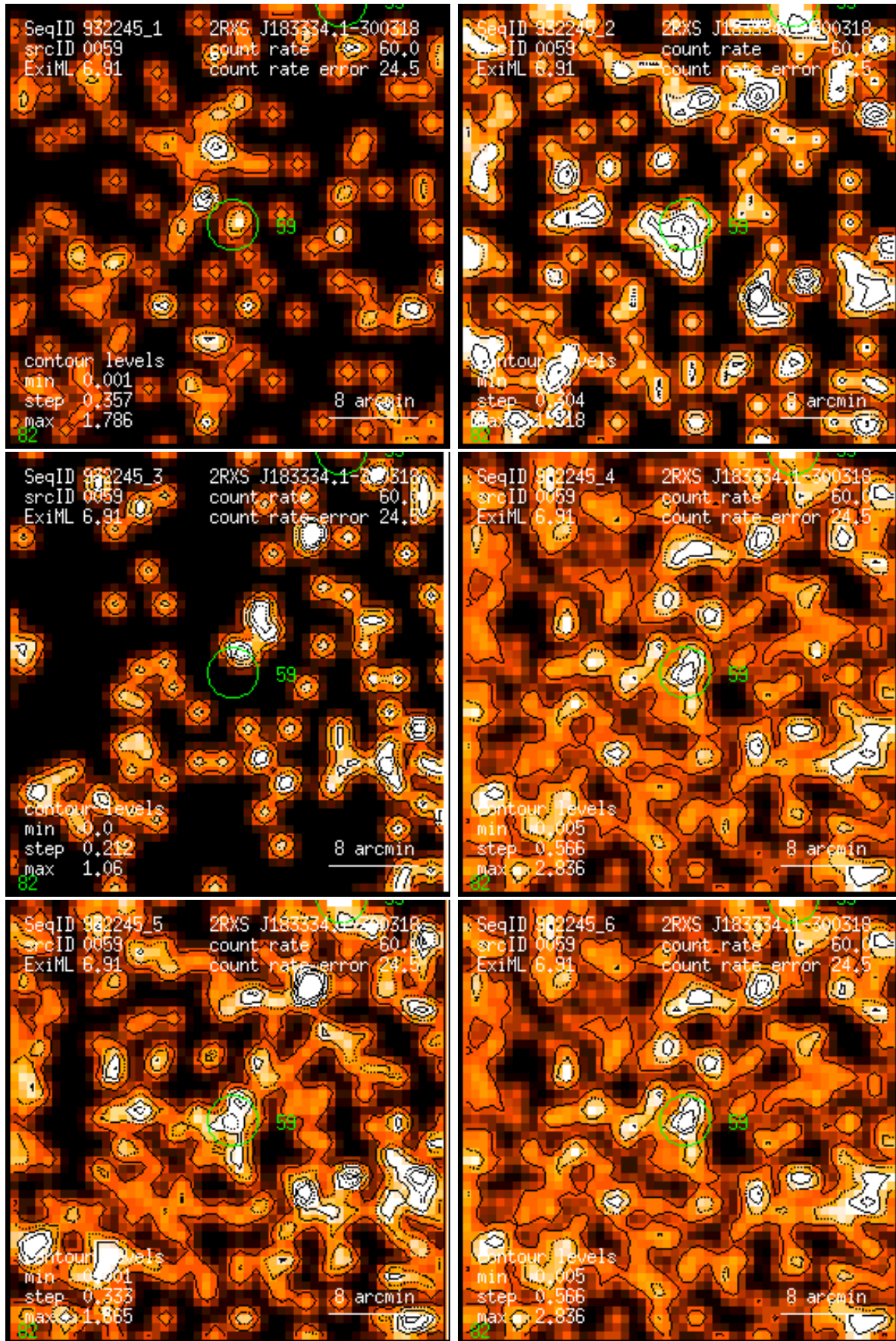
Figure 59: RASS 932245: detection 0059: band rate images, Gaussian filter: (1) PSPC channels 11 – 41, (2) 52 – 90, (3) 91 – 201, (4) 11 – 235, (5) 52 – 201, (6) 11 – 201. Broad band rates in counts/ks. Band rate contour levels in counts/ks/arcmin 2 .
