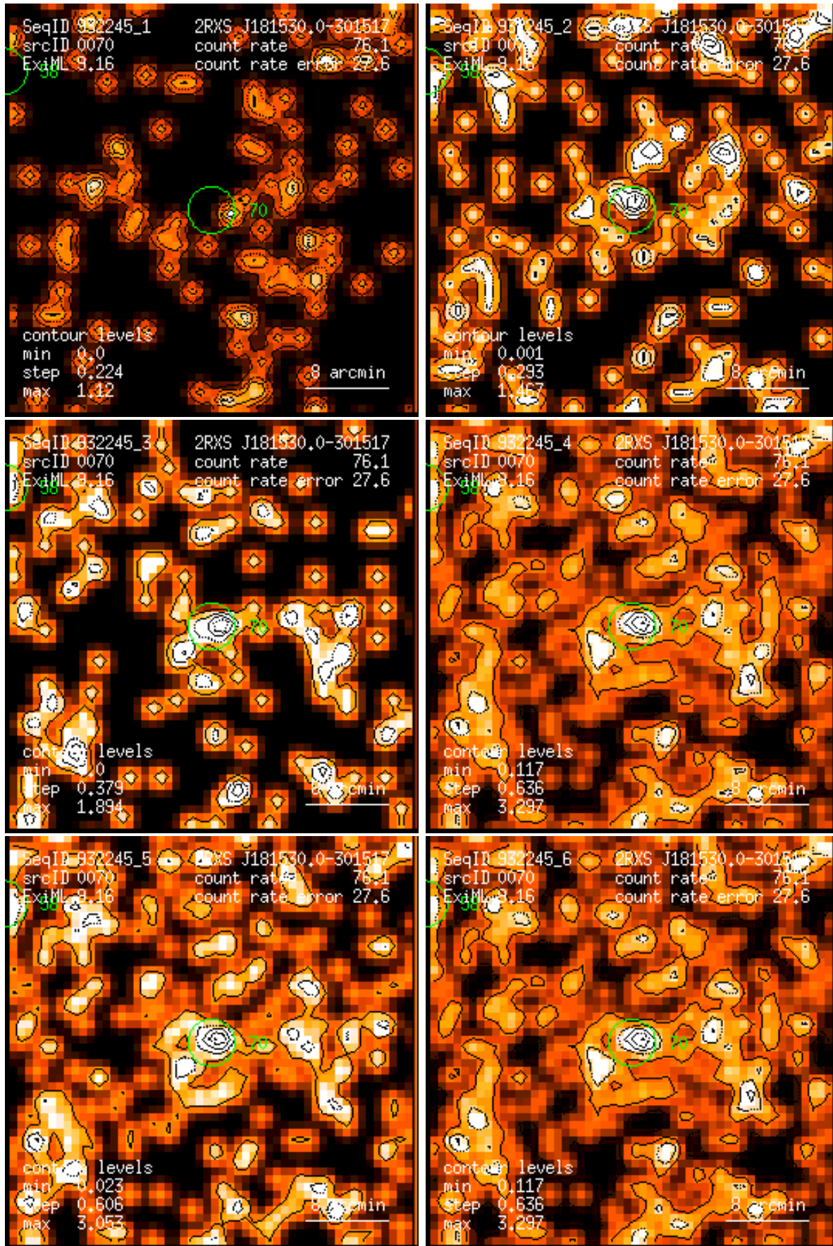
Figure 70: RASS 932245: detection 0070: band rate images, Gaussian filter: (1) PSPC channels 11 – 41, (2) 52 – 90, (3) 91 – 201, (4) 11 – 235, (5) 52 – 201, (6) 11 – 201. Broad band rates in counts/ks. Band rate contour levels in counts/ks/arcmin 2 .
