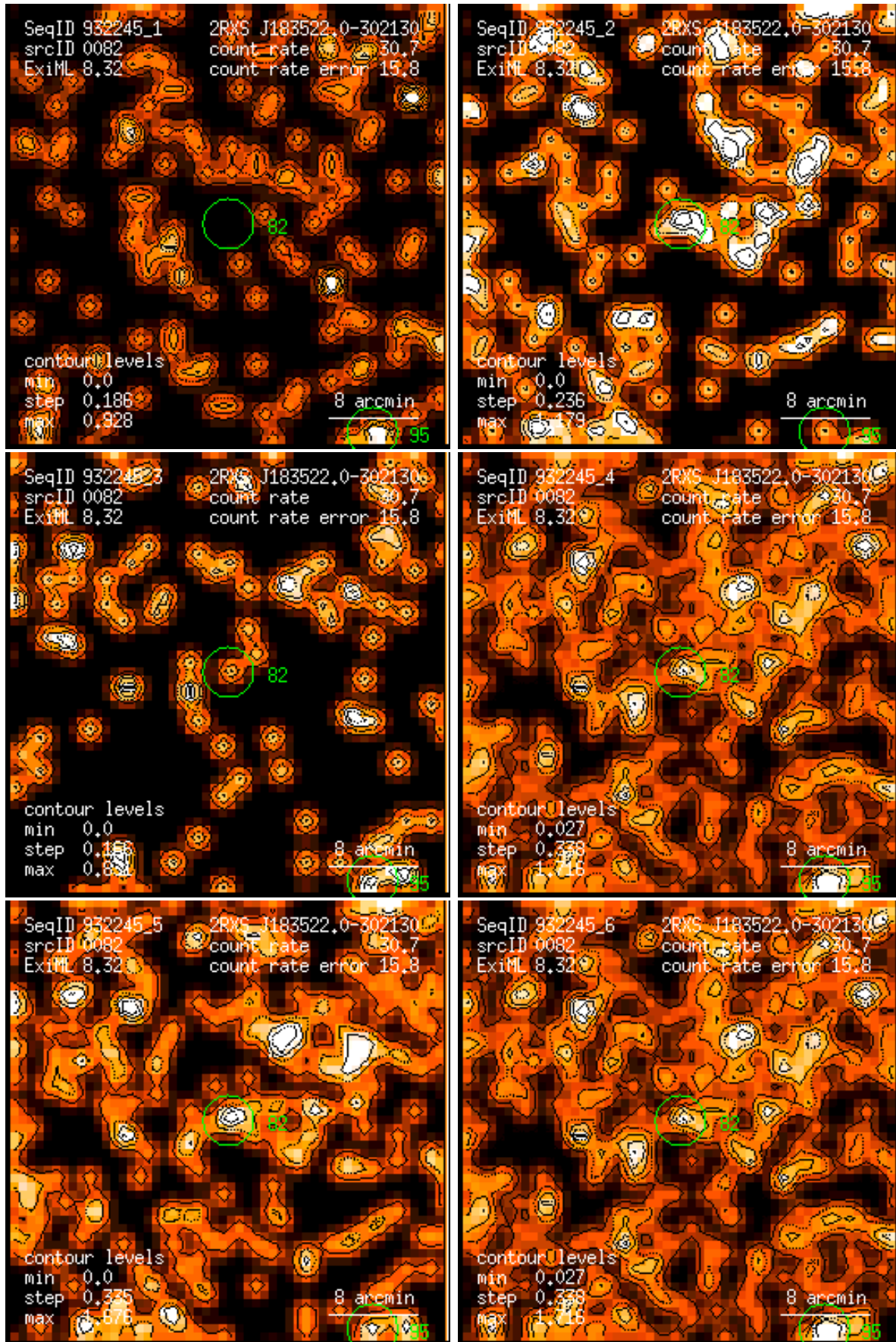
Figure 82: RASS 932245: detection 0082: band rate images, Gaussian filter: (1) PSPC channels 11 – 41, (2) 52 – 90, (3) 91 – 201, (4) 11 – 235, (5) 52 – 201, (6) 11 – 201. Broad band rates in counts/ks. Band rate contour levels in counts/ks/arcmin 2 .
