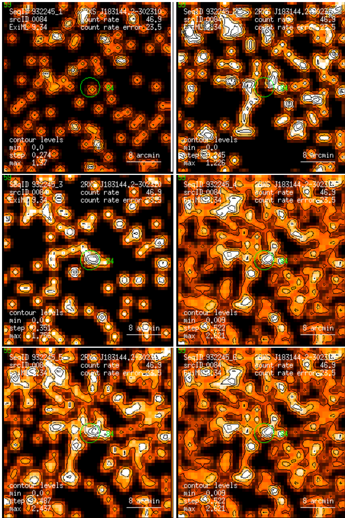
Figure 84: RASS 932245: detection 0084: band rate images, Gaussian filter: (1) PSPC channels 11 – 41, (2) 52 – 90, (3) 91 – 201, (4) 11 – 235, (5) 52 – 201, (6) 11 – 201. Broad band rates in counts/ks. Band rate contour levels in counts/ks/arcmin 2 .
