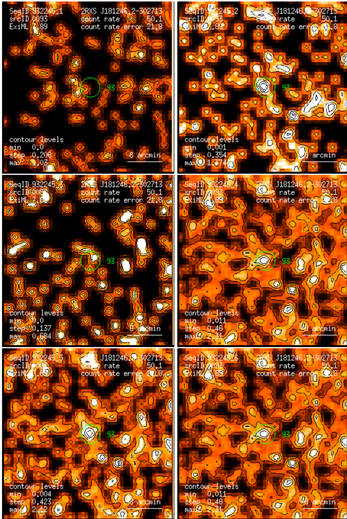
Figure 93: RASS 932245: detection 0093: band rate images, Gaussian filter: (1) PSPC channels 11 – 41, (2) 52 – 90, (3) 91 – 201, (4) 11 – 235, (5) 52 – 201, (6) 11 – 201. Broad band rates in counts/ks. Band rate contour levels in counts/ks/arcmin 2 .
