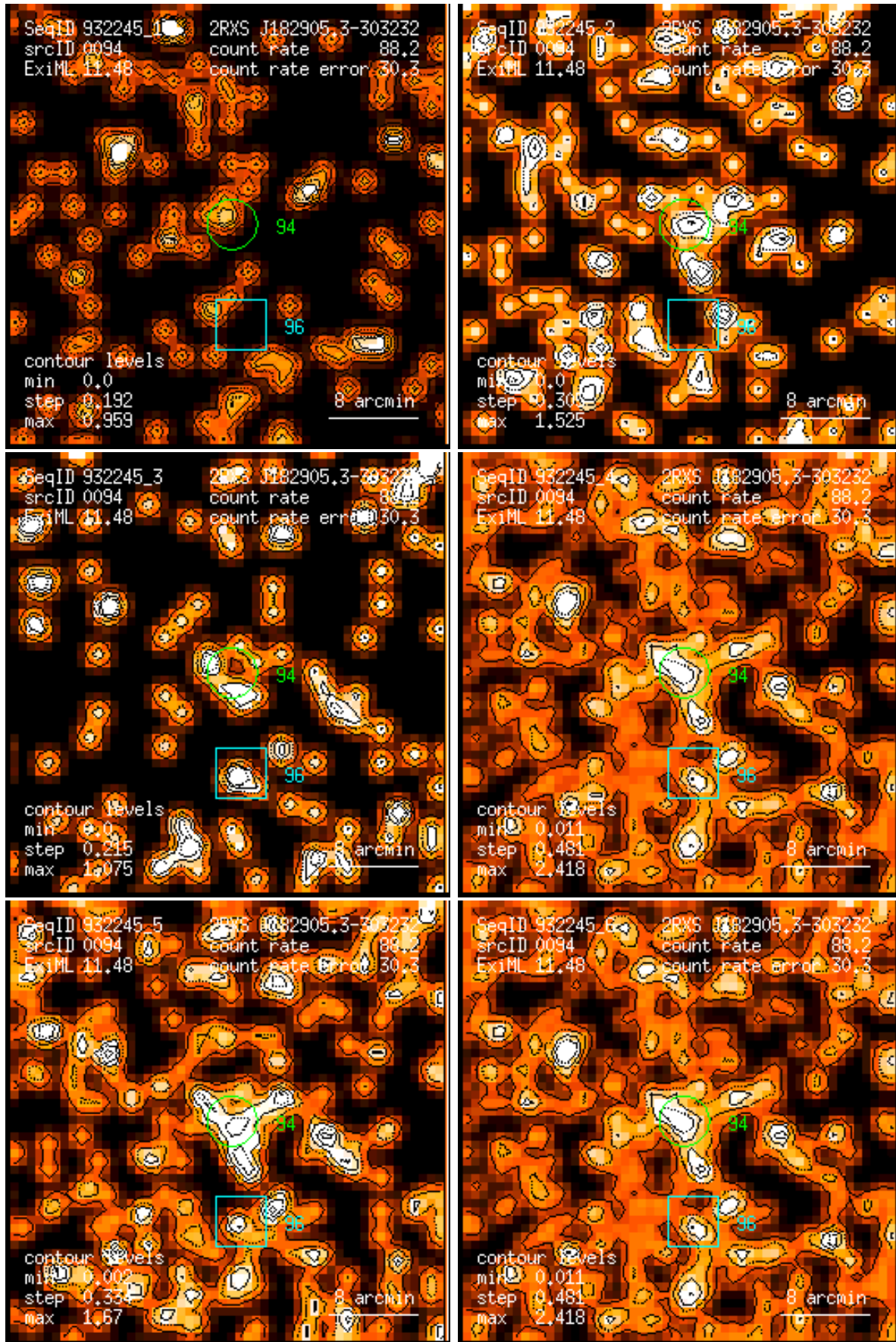
Figure 94: RASS 932245: detection 0094: band rate images, Gaussian filter: (1) PSPC channels 11 – 41, (2) 52 – 90, (3) 91 – 201, (4) 11 – 235, (5) 52 – 201, (6) 11 – 201. Broad band rates in counts/ks. Band rate contour levels in counts/ks/arcmin 2 .
