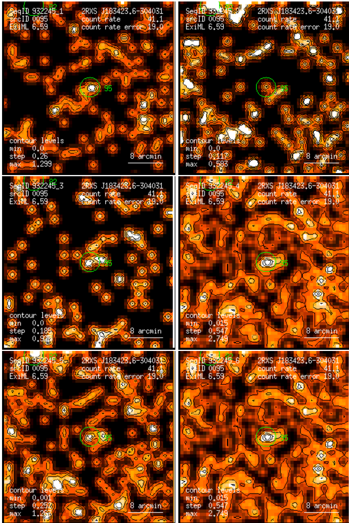
Figure 95: RASS 932245: detection 0095: band rate images, Gaussian filter: (1) PSPC channels 11 – 41, (2) 52 – 90, (3) 91 – 201, (4) 11 – 235, (5) 52 – 201, (6) 11 – 201. Broad band rates in counts/ks. Band rate contour levels in counts/ks/arcmin 2 .
