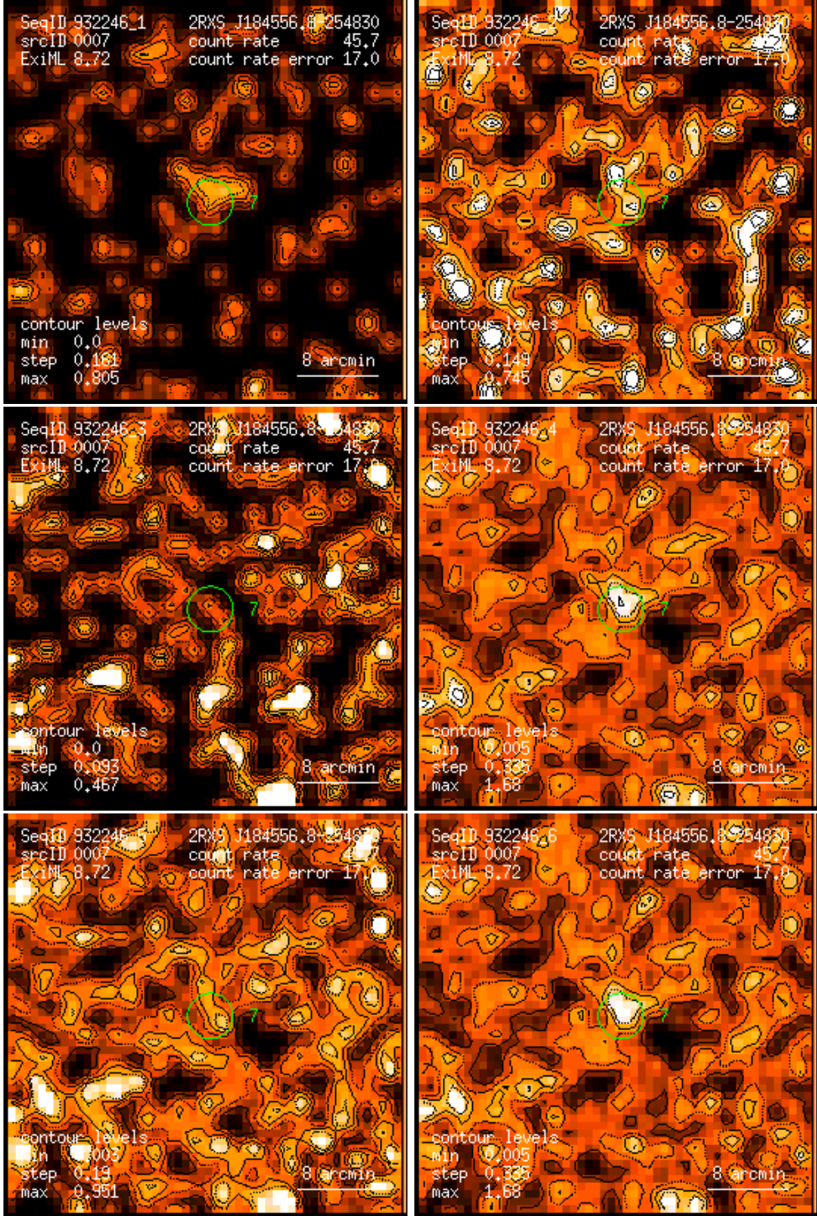
Figure 7: RASS 932246: detection 0007: band rate images, Gaussian filter: (1) PSPC channels 11 – 41, (2) 52 – 90, (3) 91 – 201, (4) 11 – 235, (5) 52 – 201, (6) 11 – 201. Broad band rates in counts/ks. Band rate contour levels in counts/ks/arcmin 2 .
