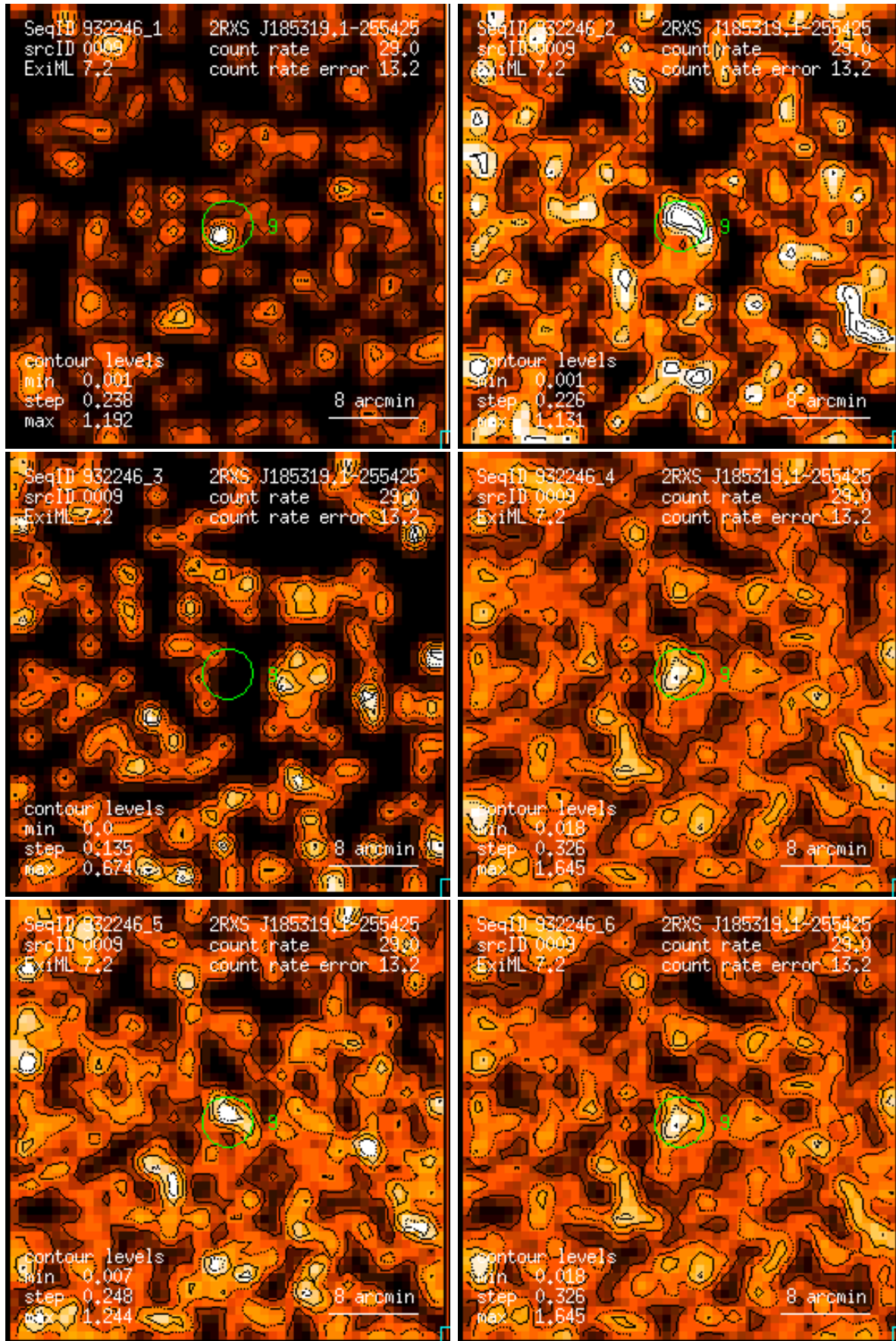
Figure 9: RASS 932246: detection 0009: band rate images, Gaussian filter: (1) PSPC channels 11 – 41, (2) 52 – 90, (3) 91 – 201, (4) 11 – 235, (5) 52 – 201, (6) 11 – 201. Broad band rates in counts/ks. Band rate contour levels in counts/ks/arcmin 2 .
