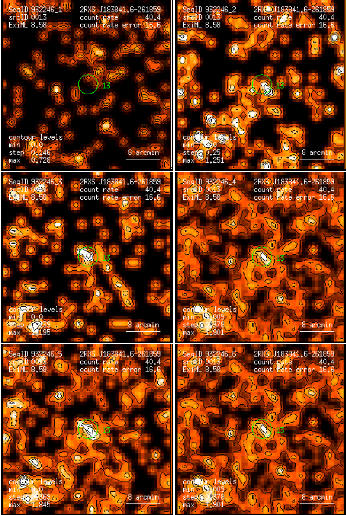
Figure 13: RASS 932246: detection 0013: band rate images, Gaussian filter: (1) PSPC channels 11 – 41, (2) 52 – 90, (3) 91 – 201, (4) 11 – 235, (5) 52 – 201, (6) 11 – 201. Broad band rates in counts/ks. Band rate contour levels in counts/ks/arcmin 2 .
