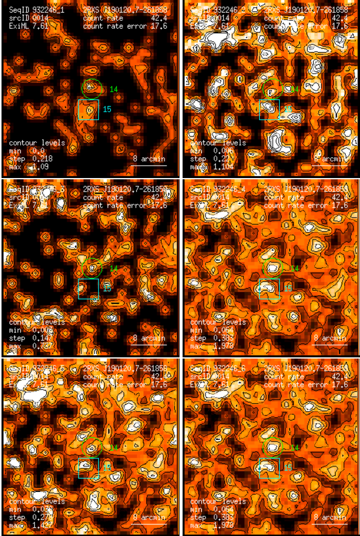
Figure 14: RASS 932246: detection 0014: band rate images, Gaussian filter: (1) PSPC channels 11 – 41, (2) 52 – 90, (3) 91 – 201, (4) 11 – 235, (5) 52 – 201, (6) 11 – 201. Broad band rates in counts/ks. Band rate contour levels in counts/ks/arcmin 2 .
