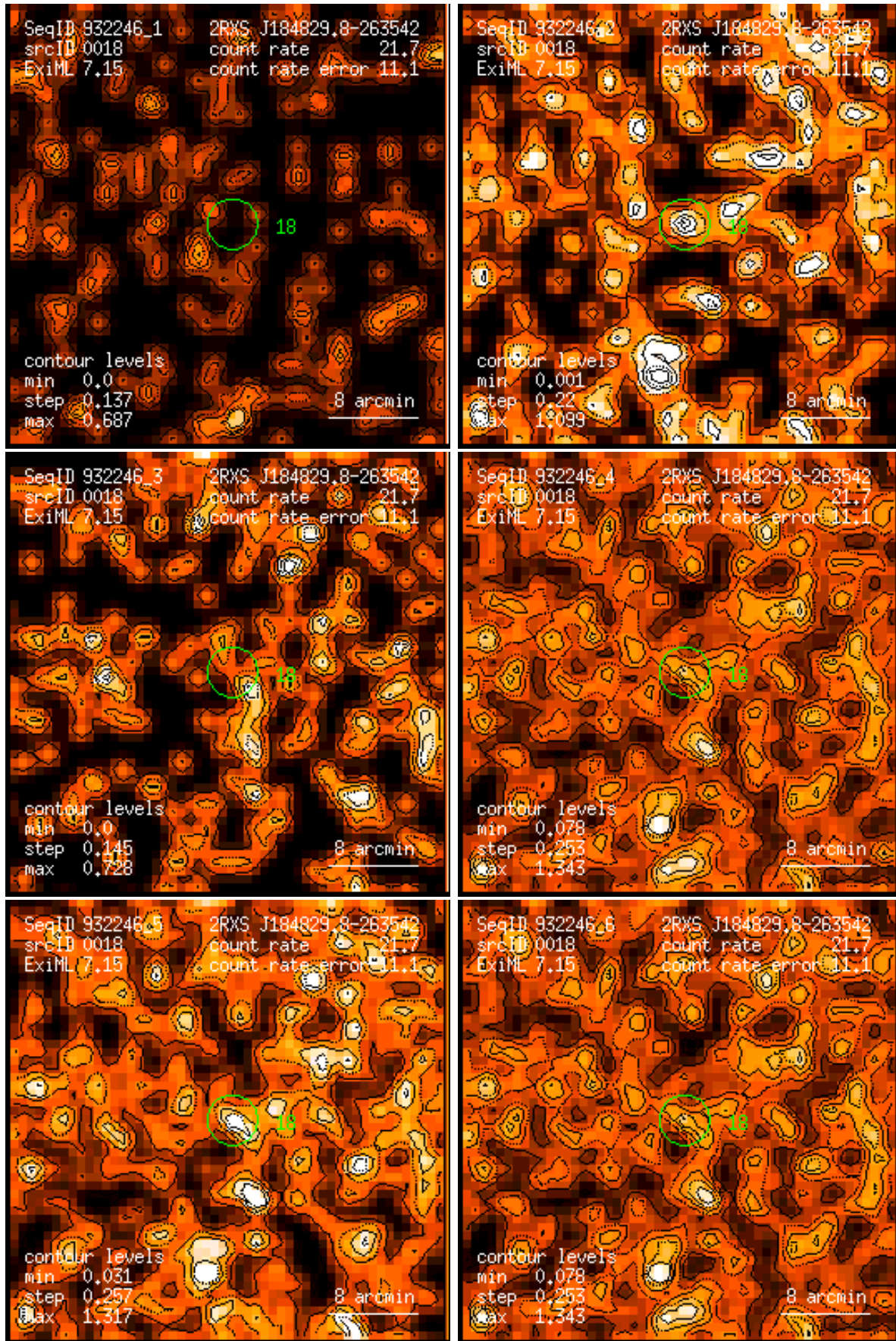
Figure 18: RASS 932246: detection 0018: band rate images, Gaussian filter: (1) PSPC channels 11 – 41, (2) 52 – 90, (3) 91 – 201, (4) 11 – 235, (5) 52 – 201, (6) 11 – 201. Broad band rates in counts/ks. Band rate contour levels in counts/ks/arcmin 2 .
