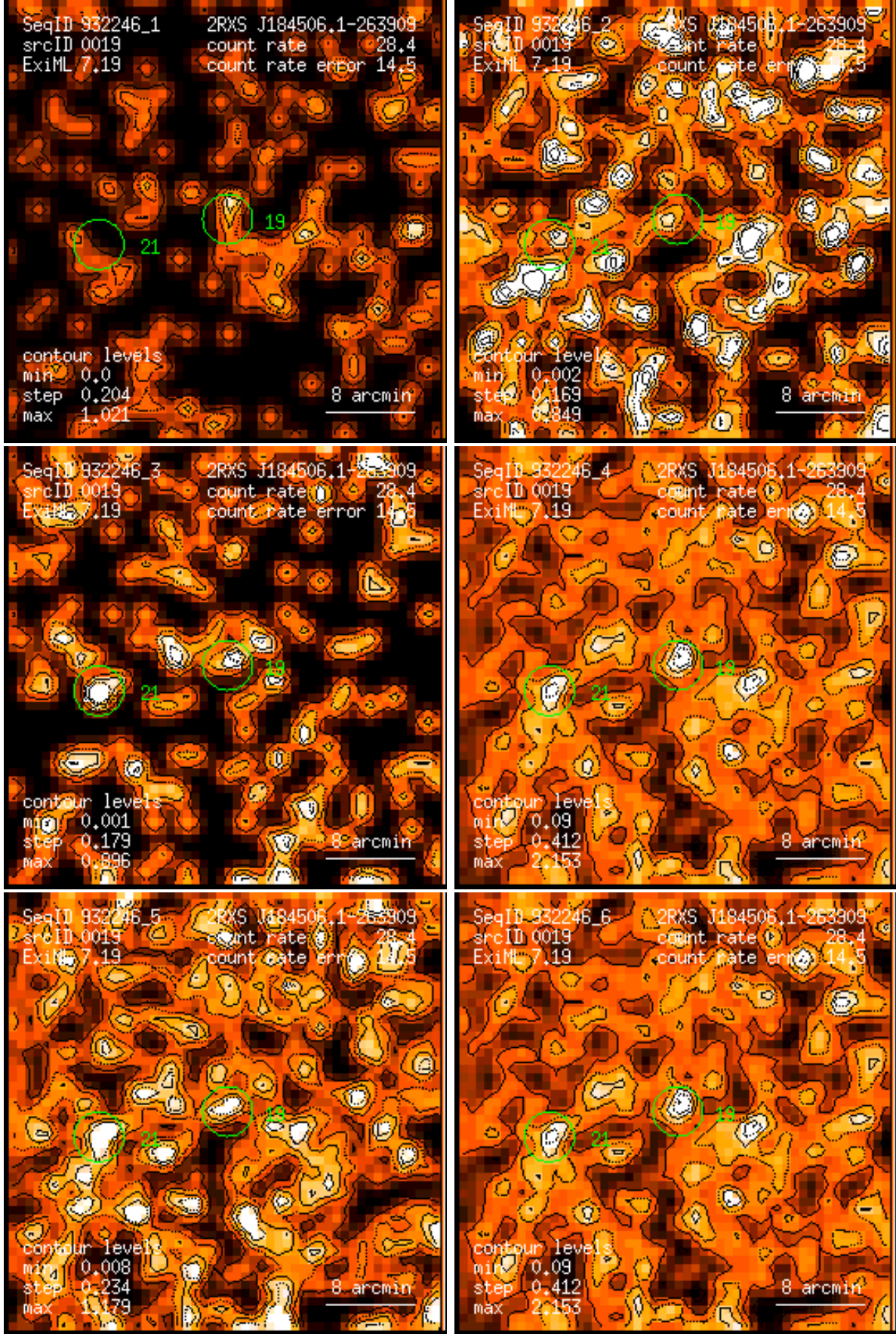
Figure 19: RASS 932246: detection 0019: band rate images, Gaussian filter: (1) PSPC channels 11 – 41, (2) 52 – 90, (3) 91 – 201, (4) 11 – 235, (5) 52 – 201, (6) 11 – 201. Broad band rates in counts/ks. Band rate contour levels in counts/ks/arcmin 2 .
