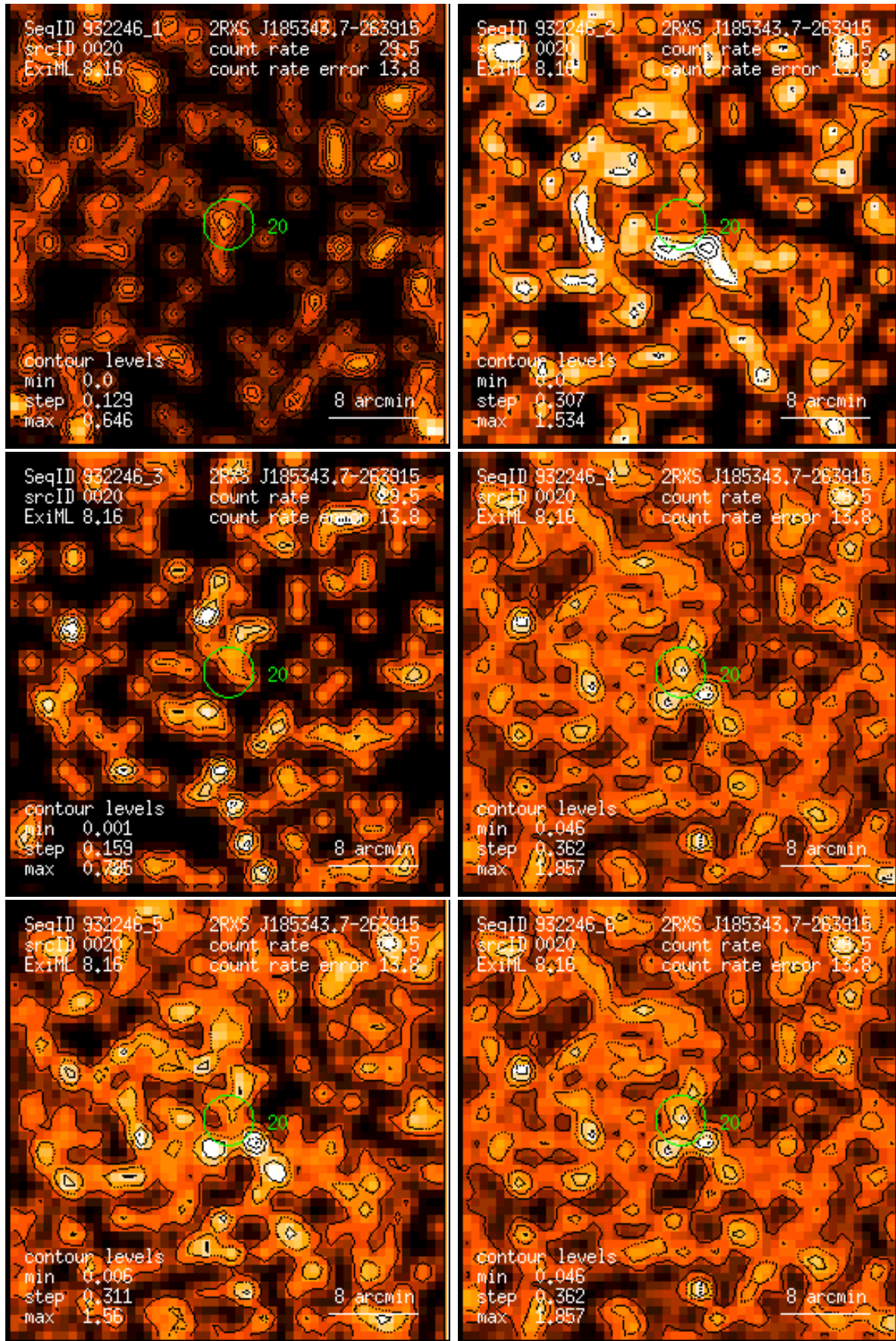
Figure 20: RASS 932246: detection 0020: band rate images, Gaussian filter: (1) PSPC channels 11 – 41, (2) 52 – 90, (3) 91 – 201, (4) 11 – 235, (5) 52 – 201, (6) 11 – 201. Broad band rates in counts/ks. Band rate contour levels in counts/ks/arcmin 2 .
