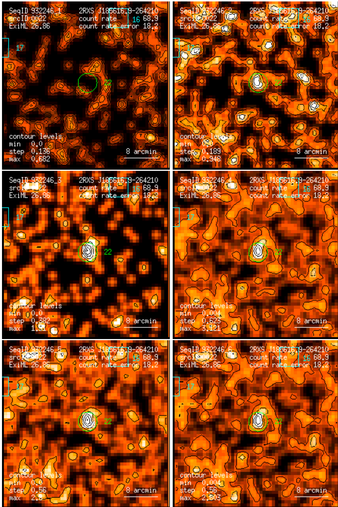
Figure 22: RASS 932246: detection 0022: band rate images, Gaussian filter: (1) PSPC channels 11 – 41, (2) 52 – 90, (3) 91 – 201, (4) 11 – 235, (5) 52 – 201, (6) 11 – 201. Broad band rates in counts/ks. Band rate contour levels in counts/ks/arcmin 2 .
