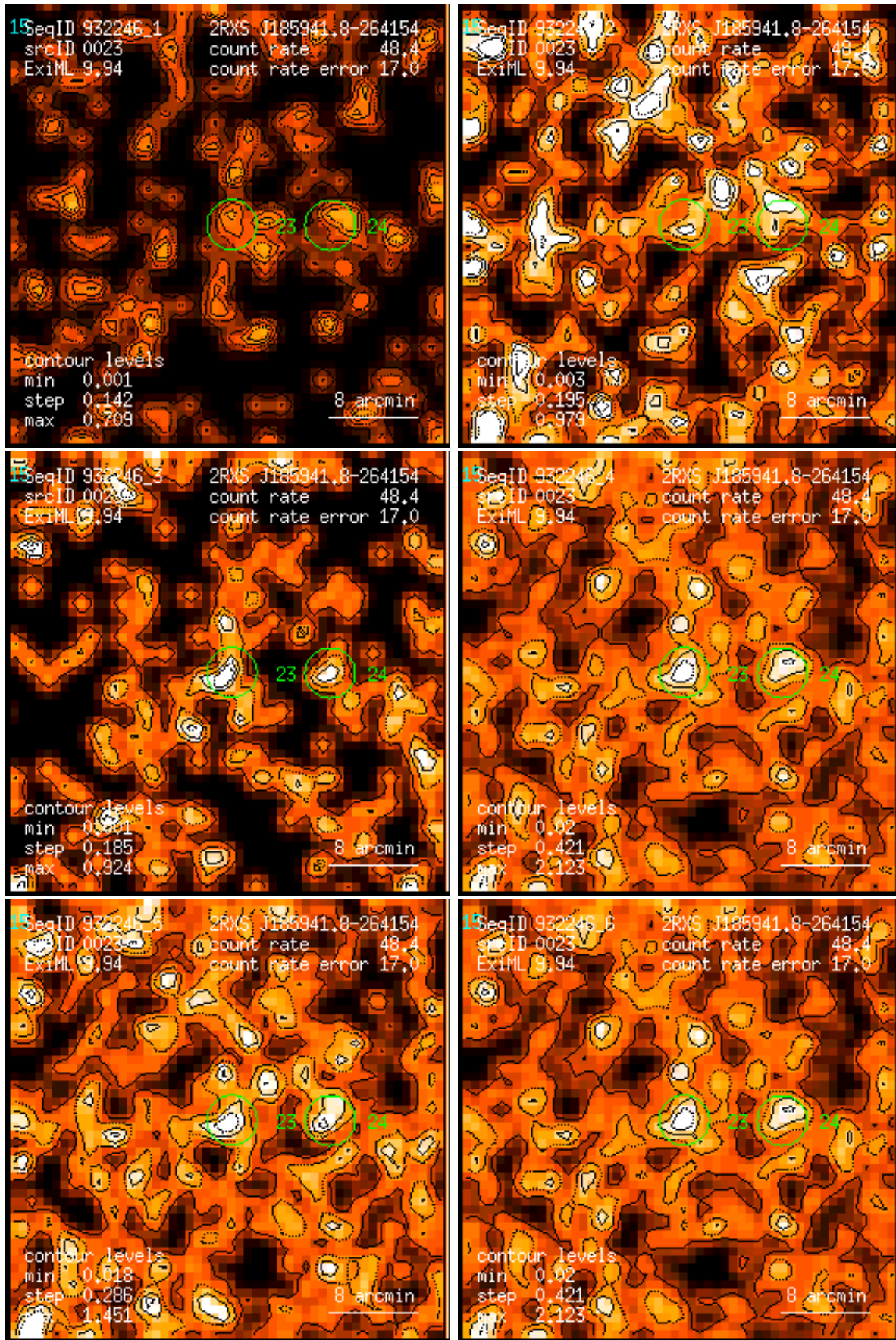
Figure 23: RASS 932246: detection 0023: band rate images, Gaussian filter: (1) PSPC channels 11 – 41, (2) 52 – 90, (3) 91 – 201, (4) 11 – 235, (5) 52 – 201, (6) 11 – 201. Broad band rates in counts/ks. Band rate contour levels in counts/ks/arcmin 2 .
