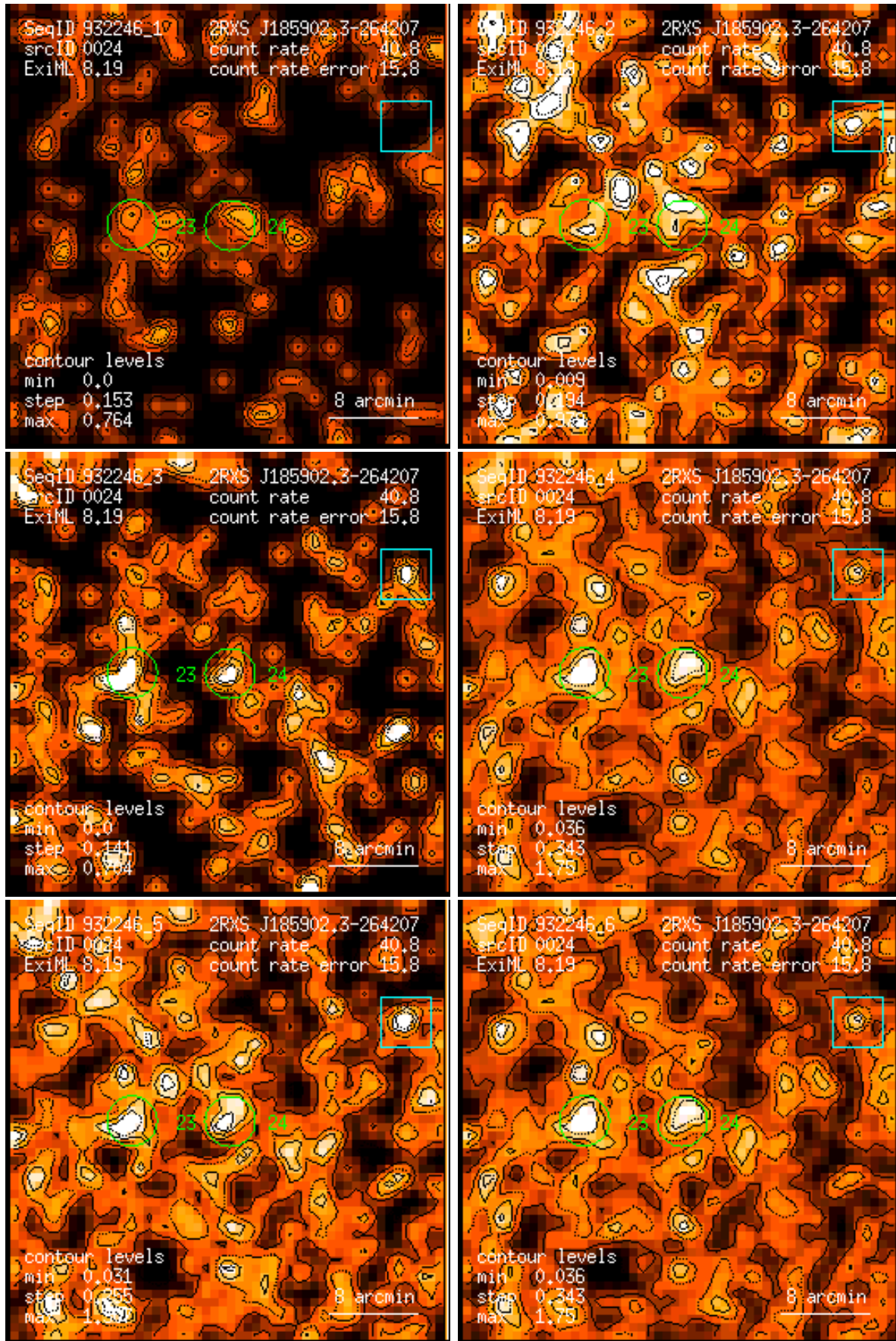
Figure 24: RASS 932246: detection 0024: band rate images, Gaussian filter: (1) PSPC channels 11 – 41, (2) 52 – 90, (3) 91 – 201, (4) 11 – 235, (5) 52 – 201, (6) 11 – 201. Broad band rates in counts/ks. Band rate contour levels in counts/ks/arcmin 2 .
