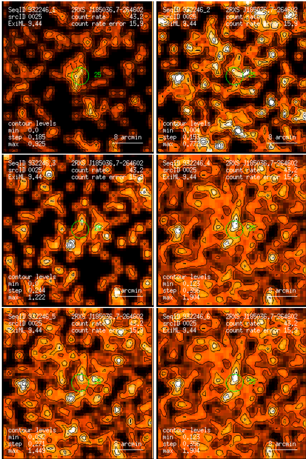
Figure 25: RASS 932246: detection 0025: band rate images, Gaussian filter: (1) PSPC channels 11 – 41, (2) 52 – 90, (3) 91 – 201, (4) 11 – 235, (5) 52 – 201, (6) 11 – 201. Broad band rates in counts/ks. Band rate contour levels in counts/ks/arcmin 2 .
