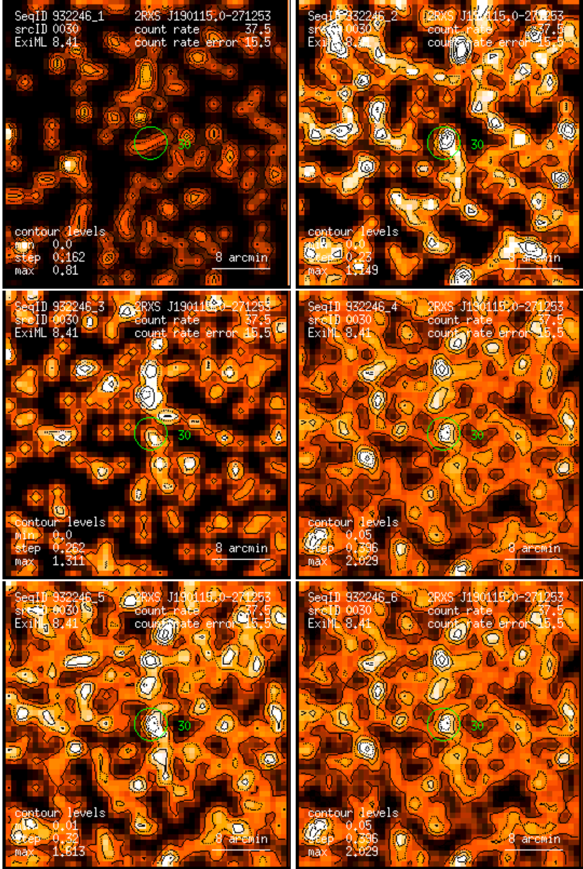
Figure 30: RASS 932246: detection 0030: band rate images, Gaussian filter: (1) PSPC channels 11 – 41, (2) 52 – 90, (3) 91 – 201, (4) 11 – 235, (5) 52 – 201, (6) 11 – 201. Broad band rates in counts/ks. Band rate contour levels in counts/ks/arcmin 2 .
