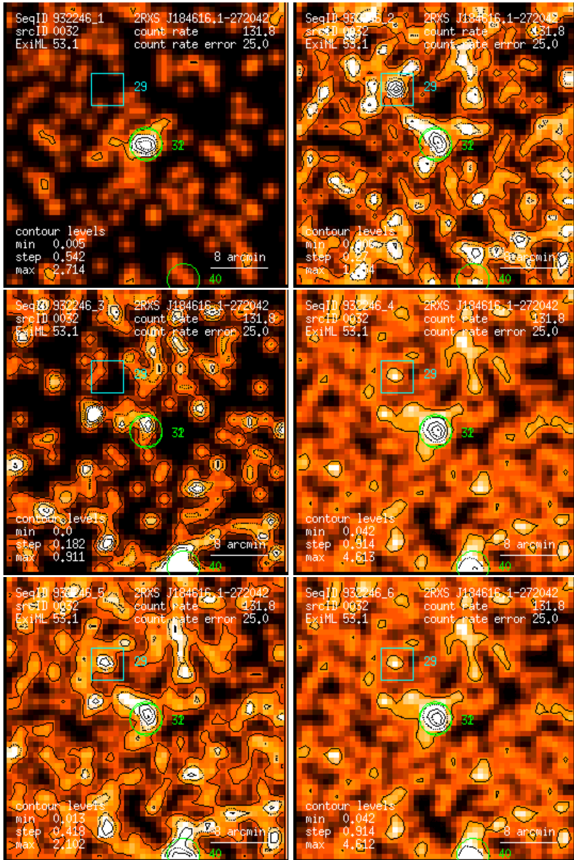
Figure 32: RASS 932246: detection 0032: band rate images, Gaussian filter: (1) PSPC channels 11 – 41, (2) 52 – 90, (3) 91 – 201, (4) 11 – 235, (5) 52 – 201, (6) 11 – 201. Broad band rates in counts/ks. Band rate contour levels in counts/ks/arcmin 2 .
