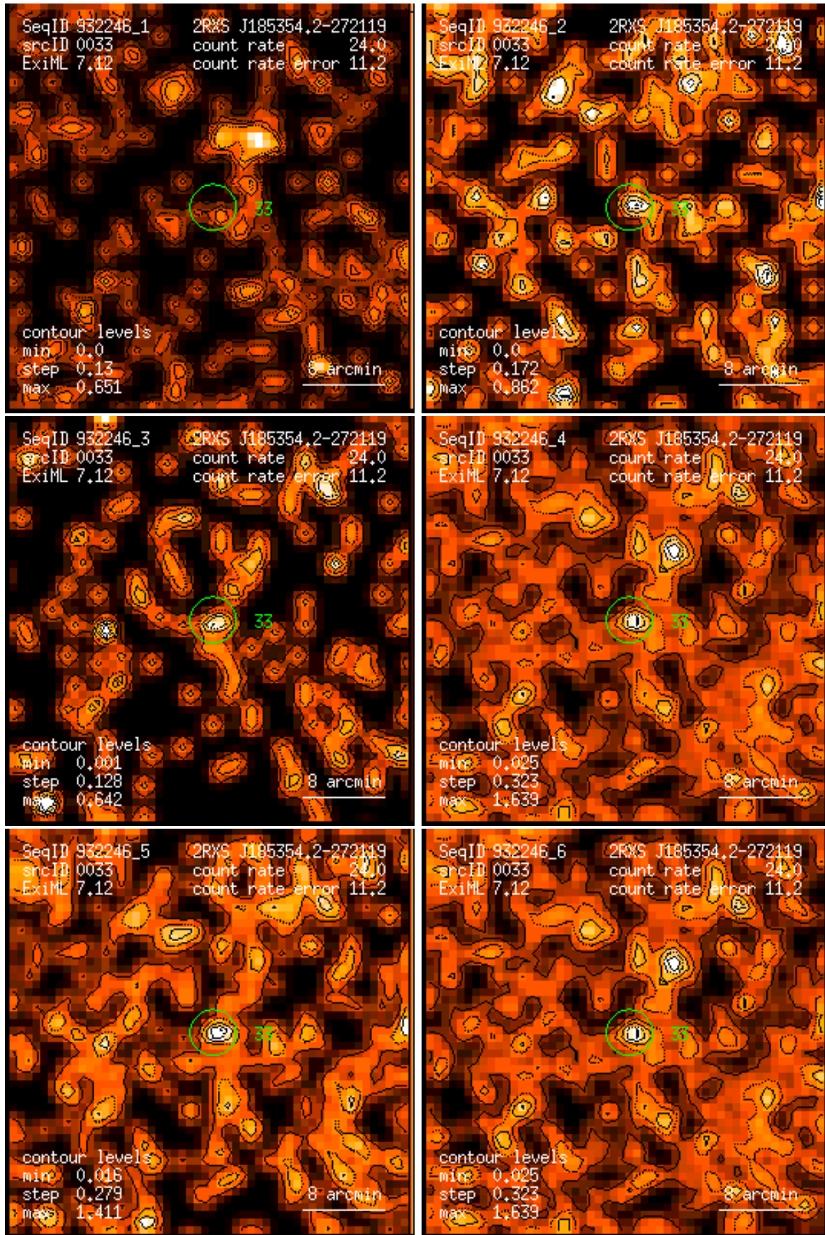
Figure 33: RASS 932246: detection 0033: band rate images, Gaussian filter: (1) PSPC channels 11 – 41, (2) 52 – 90, (3) 91 – 201, (4) 11 – 235, (5) 52 – 201, (6) 11 – 201. Broad band rates in counts/ks. Band rate contour levels in counts/ks/arcmin 2 .
