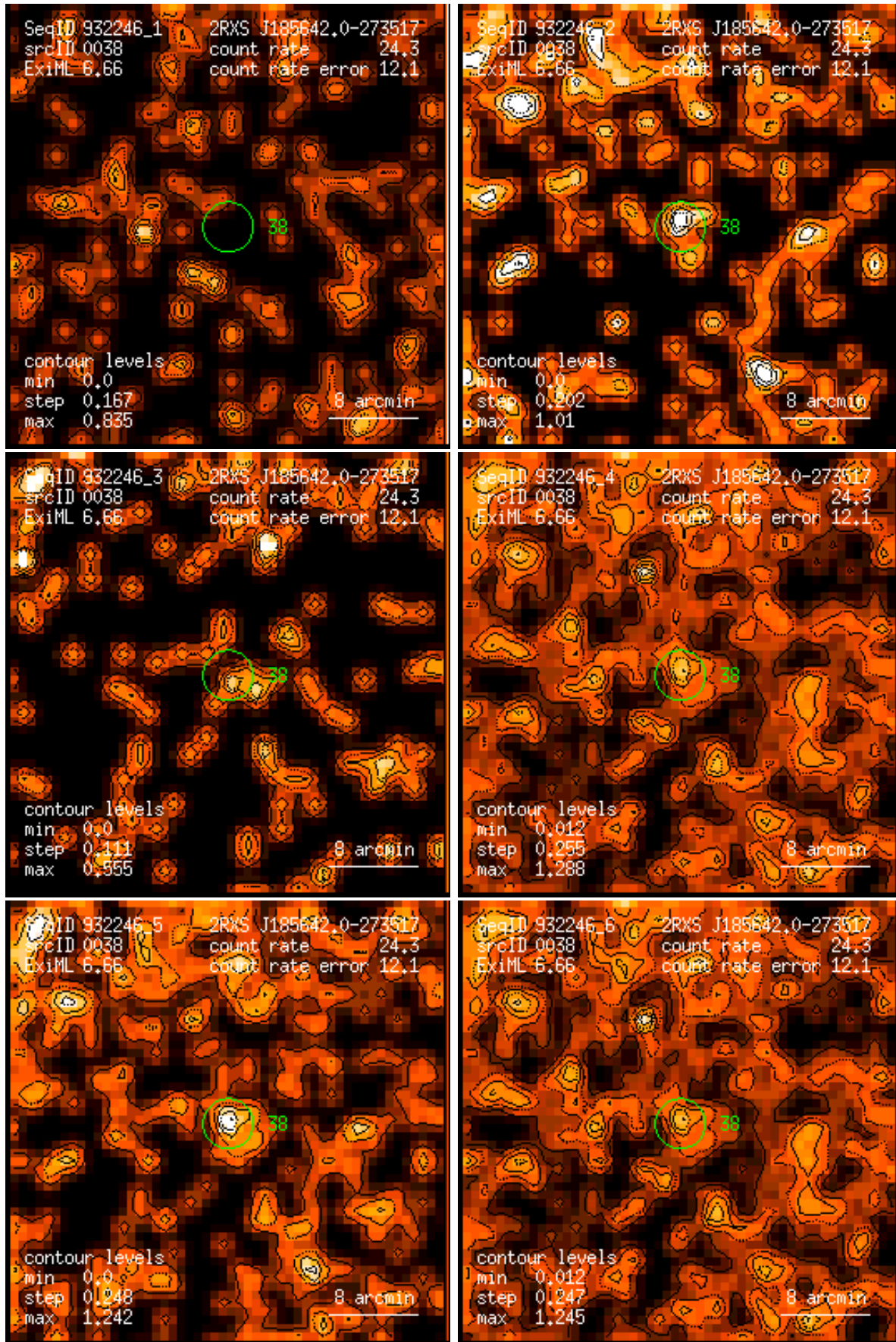
Figure 38: RASS 932246: detection 0038: band rate images, Gaussian filter: (1) PSPC channels 11 – 41, (2) 52 – 90, (3) 91 – 201, (4) 11 – 235, (5) 52 – 201, (6) 11 – 201. Broad band rates in counts/ks. Band rate contour levels in counts/ks/arcmin 2 .
