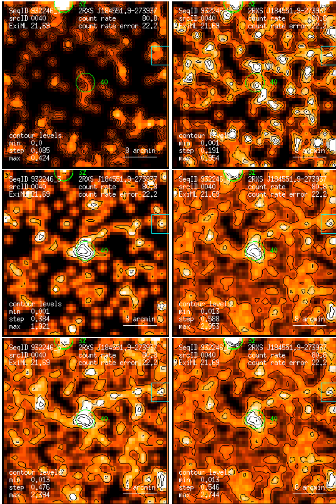
Figure 40: RASS 932246: detection 0040: band rate images, Gaussian filter: (1) PSPC channels 11 – 41, (2) 52 – 90, (3) 91 – 201, (4) 11 – 235, (5) 52 – 201, (6) 11 – 201. Broad band rates in counts/ks. Band rate contour levels in counts/ks/arcmin 2 .
