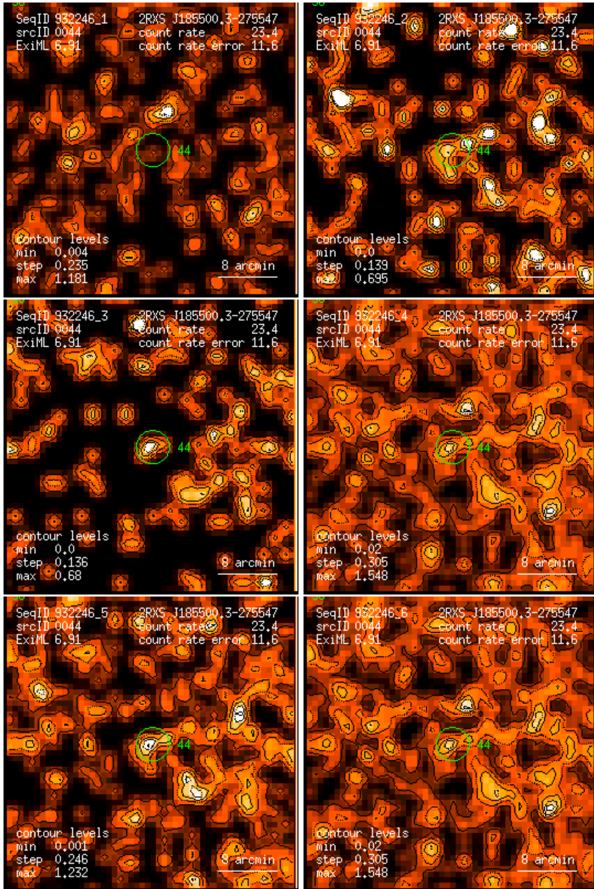
Figure 44: RASS 932246: detection 0044: band rate images, Gaussian filter: (1) PSPC channels 11 – 41, (2) 52 – 90, (3) 91 – 201, (4) 11 – 235, (5) 52 – 201, (6) 11 – 201. Broad band rates in counts/ks. Band rate contour levels in counts/ks/arcmin 2 .
