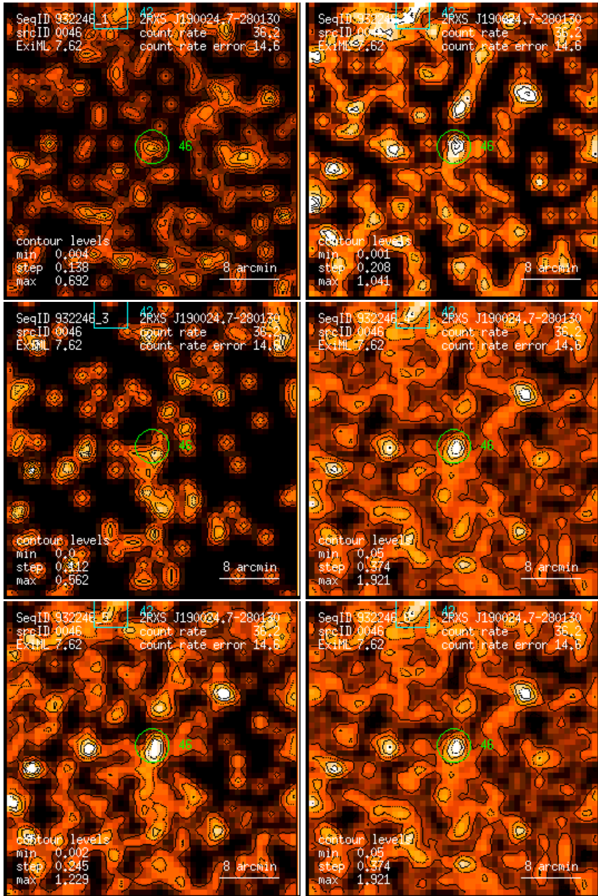
Figure 46: RASS 932246: detection 0046: band rate images, Gaussian filter: (1) PSPC channels 11 – 41, (2) 52 – 90, (3) 91 – 201, (4) 11 – 235, (5) 52 – 201, (6) 11 – 201. Broad band rates in counts/ks. Band rate contour levels in counts/ks/arcmin 2 .
