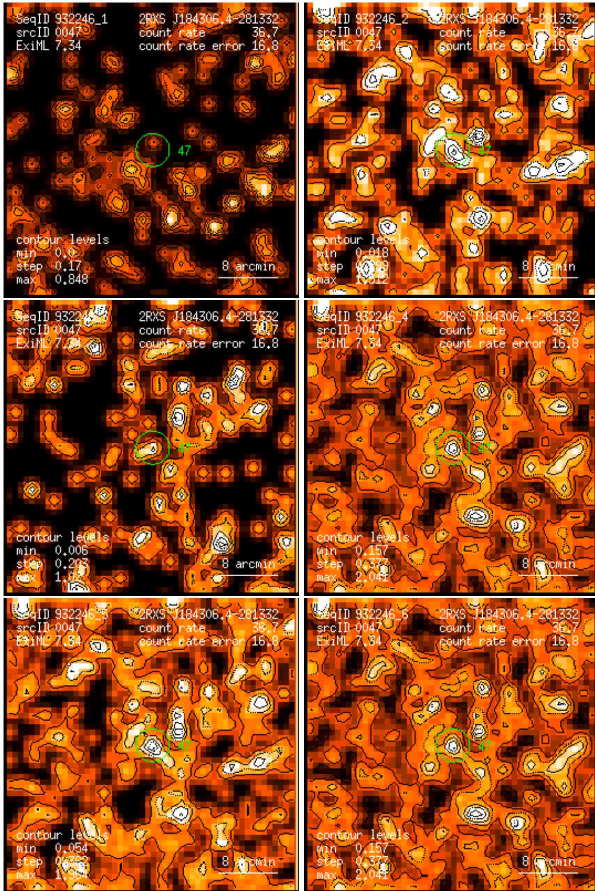
Figure 47: RASS 932246: detection 0047: band rate images, Gaussian filter: (1) PSPC channels 11 – 41, (2) 52 – 90, (3) 91 – 201, (4) 11 – 235, (5) 52 – 201, (6) 11 – 201. Broad band rates in counts/ks. Band rate contour levels in counts/ks/arcmin 2 .
