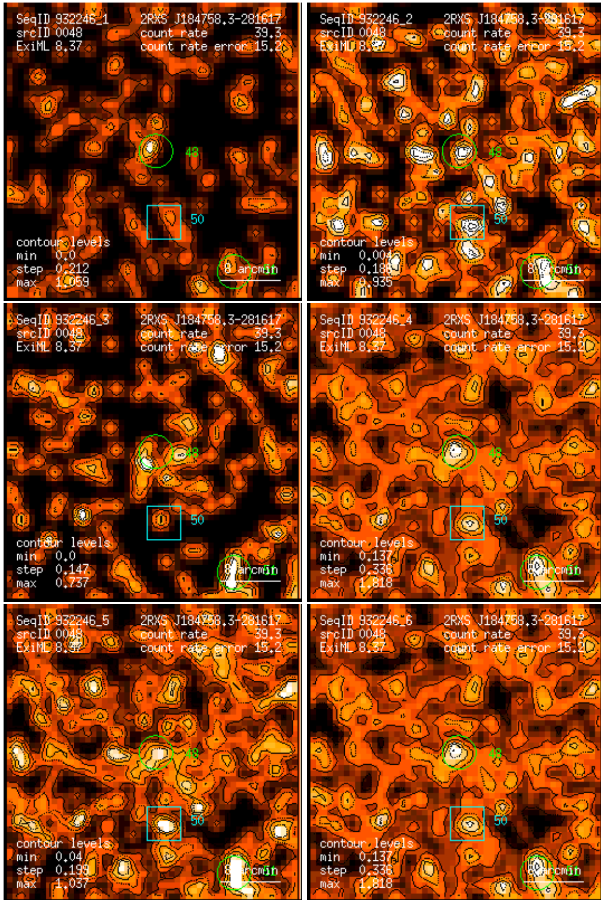
Figure 48: RASS 932246: detection 0048: band rate images, Gaussian filter: (1) PSPC channels 11 – 41, (2) 52 – 90, (3) 91 – 201, (4) 11 – 235, (5) 52 – 201, (6) 11 – 201. Broad band rates in counts/ks. Band rate contour levels in counts/ks/arcmin 2 .
