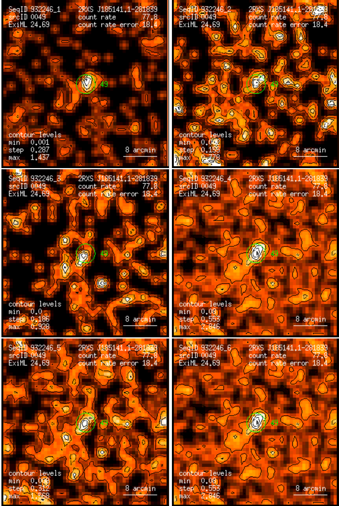
Figure 49: RASS 932246: detection 0049: band rate images, Gaussian filter: (1) PSPC channels 11 – 41, (2) 52 – 90, (3) 91 – 201, (4) 11 – 235, (5) 52 – 201, (6) 11 – 201. Broad band rates in counts/ks. Band rate contour levels in counts/ks/arcmin 2 .
