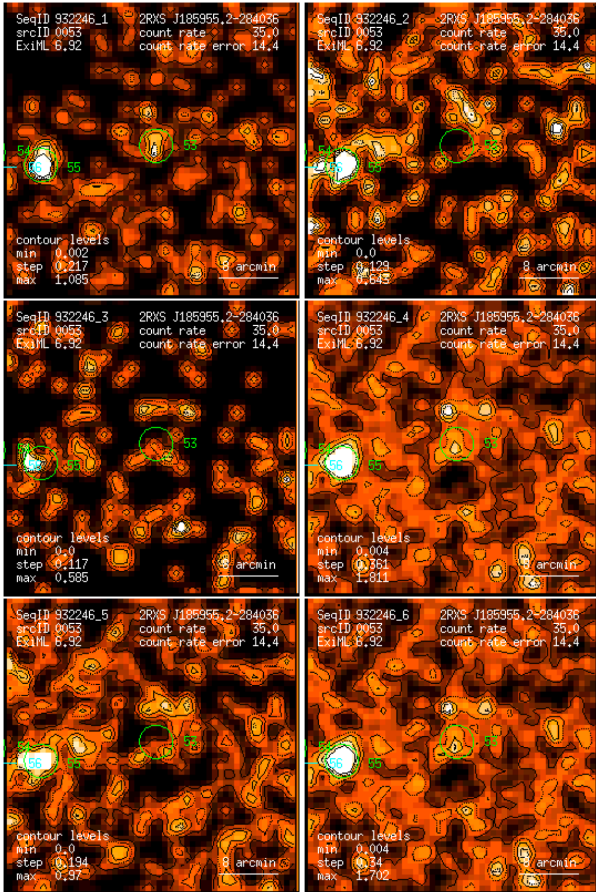
Figure 53: RASS 932246: detection 0053: band rate images, Gaussian filter: (1) PSPC channels 11 – 41, (2) 52 – 90, (3) 91 – 201, (4) 11 – 235, (5) 52 – 201, (6) 11 – 201. Broad band rates in counts/ks. Band rate contour levels in counts/ks/arcmin 2 .
