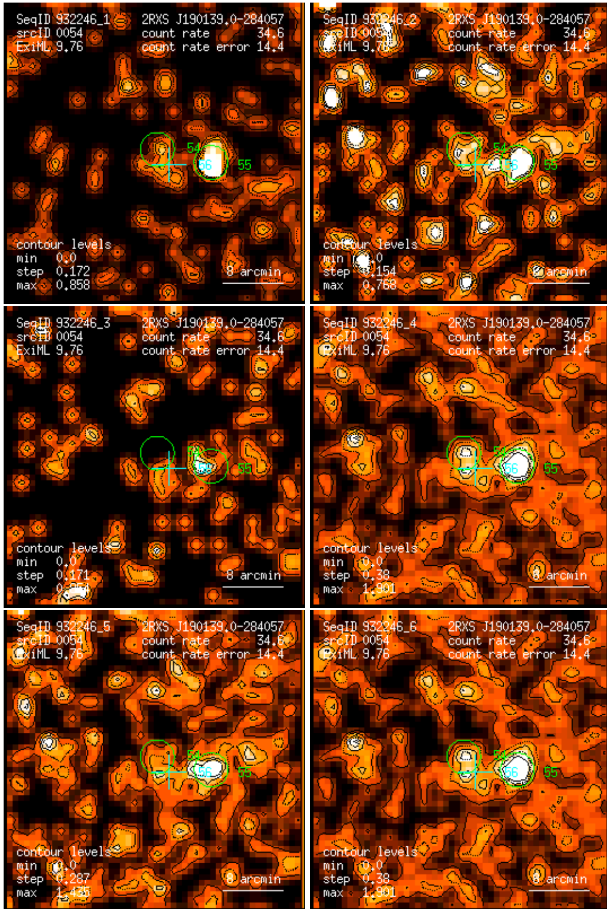
Figure 54: RASS 932246: detection 0054: band rate images, Gaussian filter: (1) PSPC channels 11 – 41, (2) 52 – 90, (3) 91 – 201, (4) 11 – 235, (5) 52 – 201, (6) 11 – 201. Broad band rates in counts/ks. Band rate contour levels in counts/ks/arcmin 2 .
