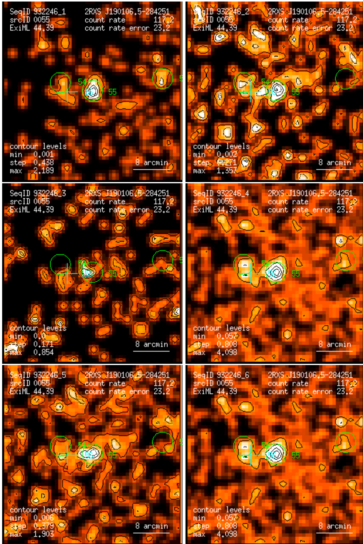
Figure 55: RASS 932246: detection 0055: band rate images, Gaussian filter: (1) PSPC channels 11 – 41, (2) 52 – 90, (3) 91 – 201, (4) 11 – 235, (5) 52 – 201, (6) 11 – 201. Broad band rates in counts/ks. Band rate contour levels in counts/ks/arcmin 2 .
