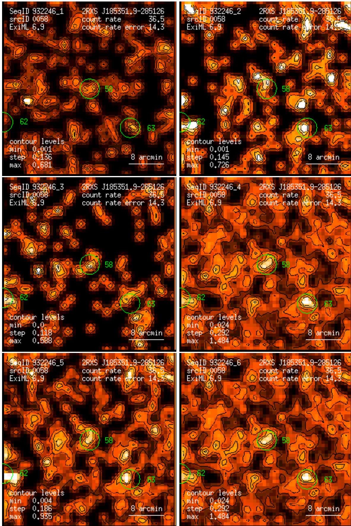
Figure 58: RASS 932246: detection 0058: band rate images, Gaussian filter: (1) PSPC channels 11 – 41, (2) 52 – 90, (3) 91 – 201, (4) 11 – 235, (5) 52 – 201, (6) 11 – 201. Broad band rates in counts/ks. Band rate contour levels in counts/ks/arcmin 2 .
