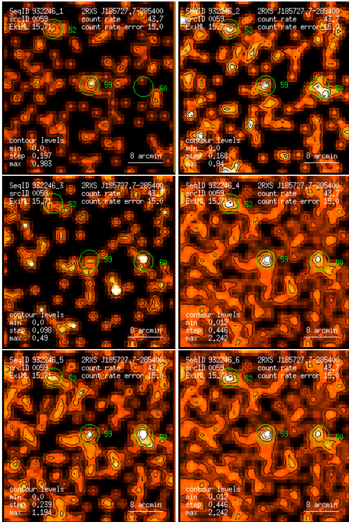
Figure 59: RASS 932246: detection 0059: band rate images, Gaussian filter: (1) PSPC channels 11 – 41, (2) 52 – 90, (3) 91 – 201, (4) 11 – 235, (5) 52 – 201, (6) 11 – 201. Broad band rates in counts/ks. Band rate contour levels in counts/ks/arcmin 2 .
