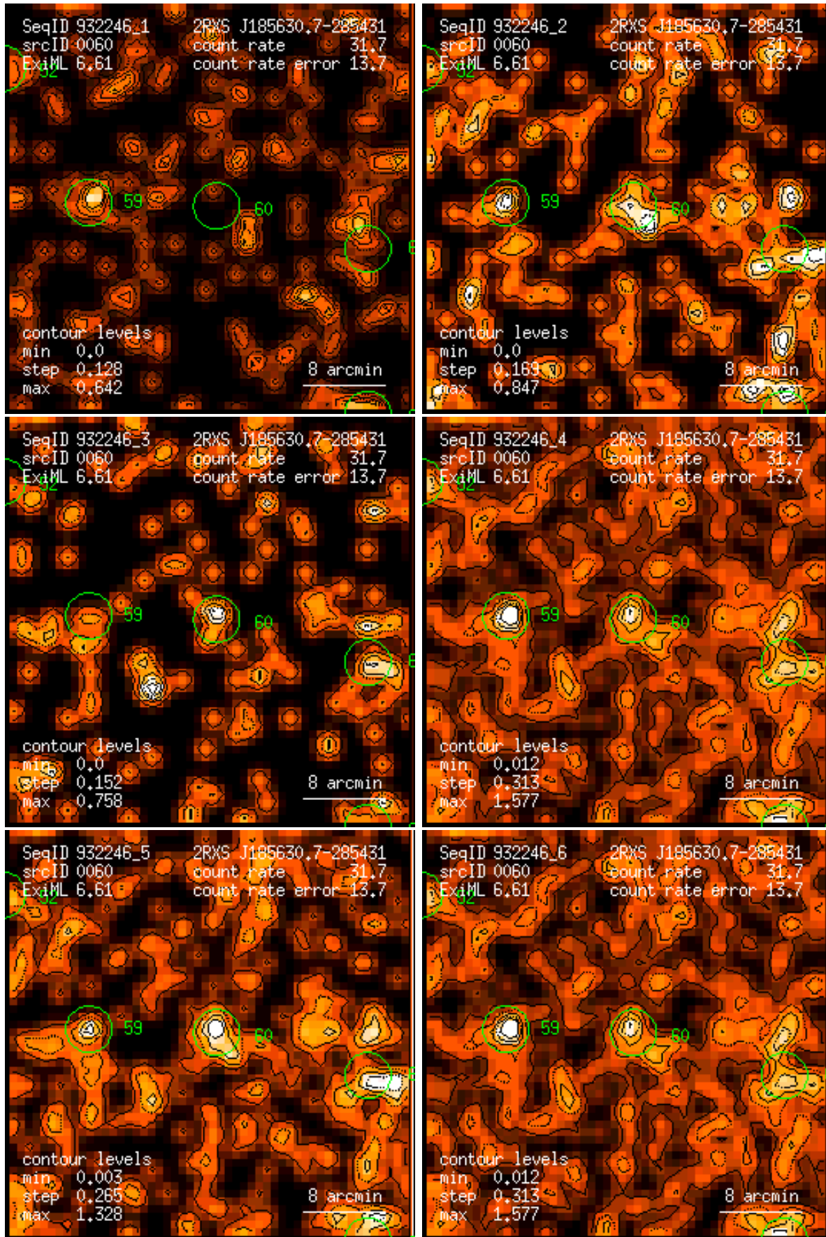
Figure 60: RASS 932246: detection 0060: band rate images, Gaussian filter: (1) PSPC channels 11 – 41, (2) 52 – 90, (3) 91 – 201, (4) 11 – 235, (5) 52 – 201, (6) 11 – 201. Broad band rates in counts/ks. Band rate contour levels in counts/ks/arcmin 2 .
