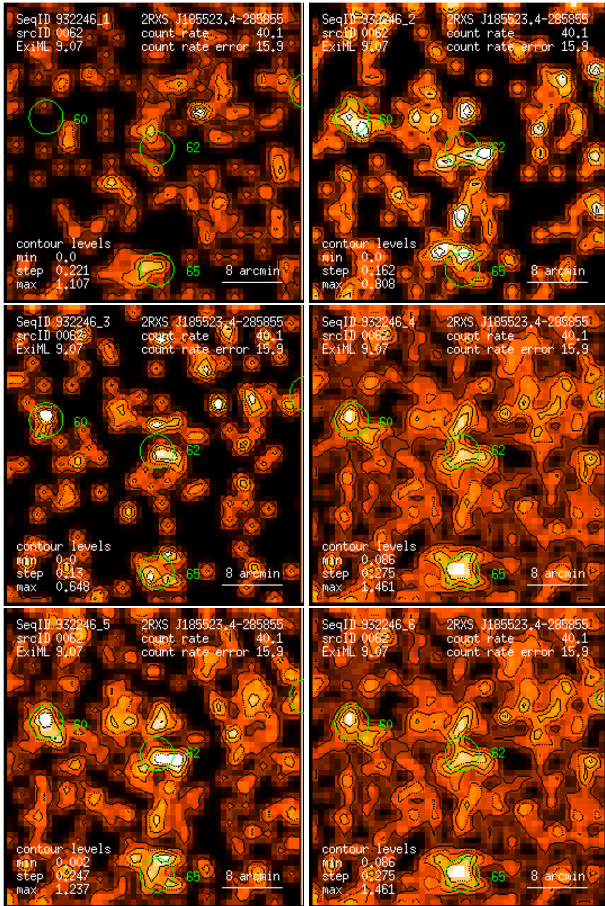
Figure 62: RASS 932246: detection 0062: band rate images, Gaussian filter: (1) PSPC channels 11 – 41, (2) 52 – 90, (3) 91 – 201, (4) 11 – 235, (5) 52 – 201, (6) 11 – 201. Broad band rates in counts/ks. Band rate contour levels in counts/ks/arcmin 2 .
