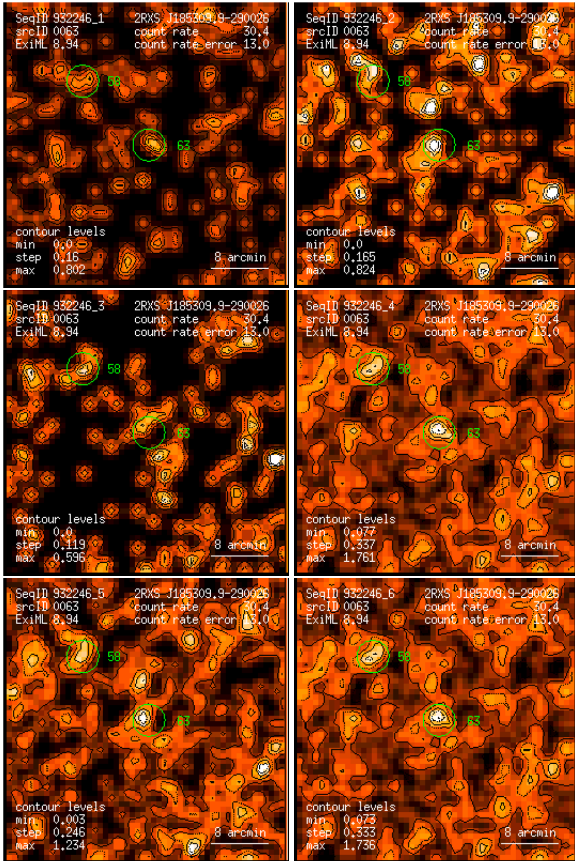
Figure 63: RASS 932246: detection 0063: band rate images, Gaussian filter: (1) PSPC channels 11 – 41, (2) 52 – 90, (3) 91 – 201, (4) 11 – 235, (5) 52 – 201, (6) 11 – 201. Broad band rates in counts/ks. Band rate contour levels in counts/ks/arcmin 2 .
