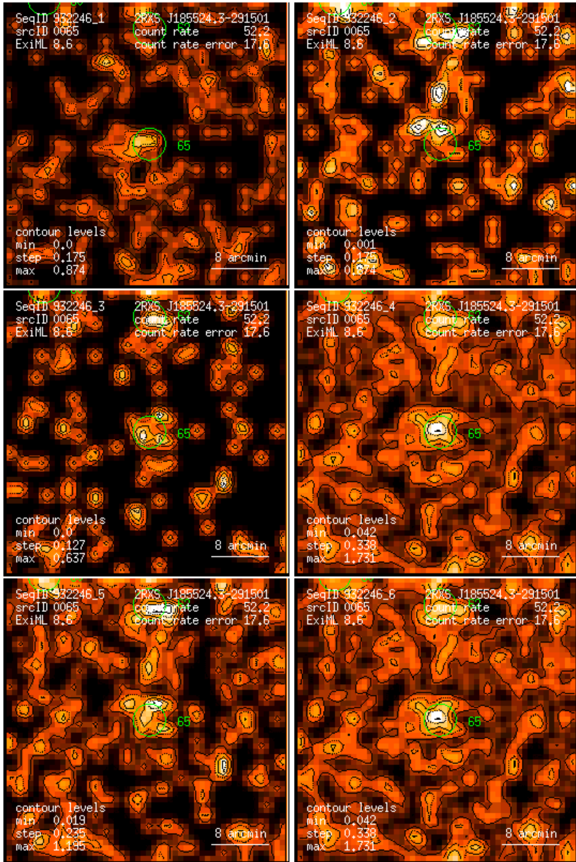
Figure 65: RASS 932246: detection 0065: band rate images, Gaussian filter: (1) PSPC channels 11 – 41, (2) 52 – 90, (3) 91 – 201, (4) 11 – 235, (5) 52 – 201, (6) 11 – 201. Broad band rates in counts/ks. Band rate contour levels in counts/ks/arcmin 2 .
