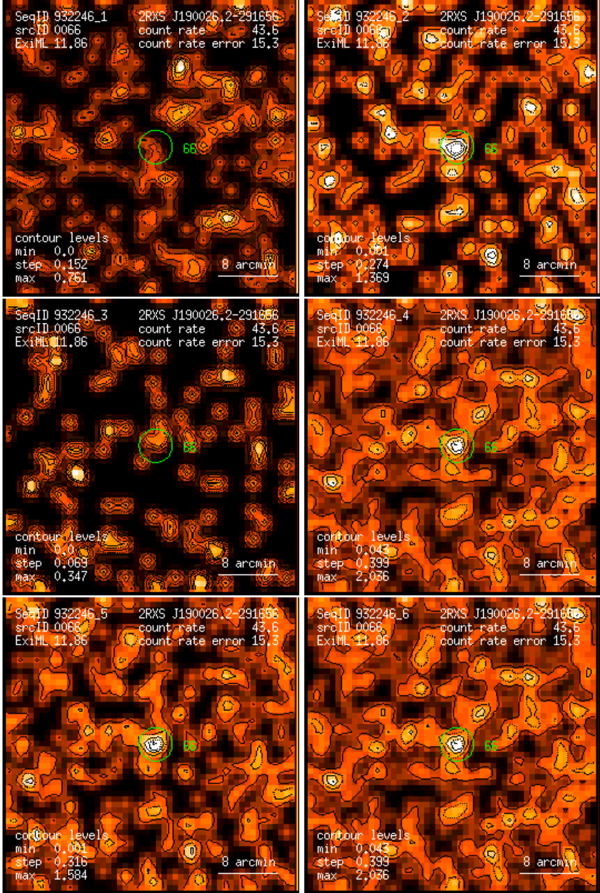
Figure 66: RASS 932246: detection 0066: band rate images, Gaussian filter: (1) PSPC channels 11 – 41, (2) 52 – 90, (3) 91 – 201, (4) 11 – 235, (5) 52 – 201, (6) 11 – 201. Broad band rates in counts/ks. Band rate contour levels in counts/ks/arcmin 2 .
