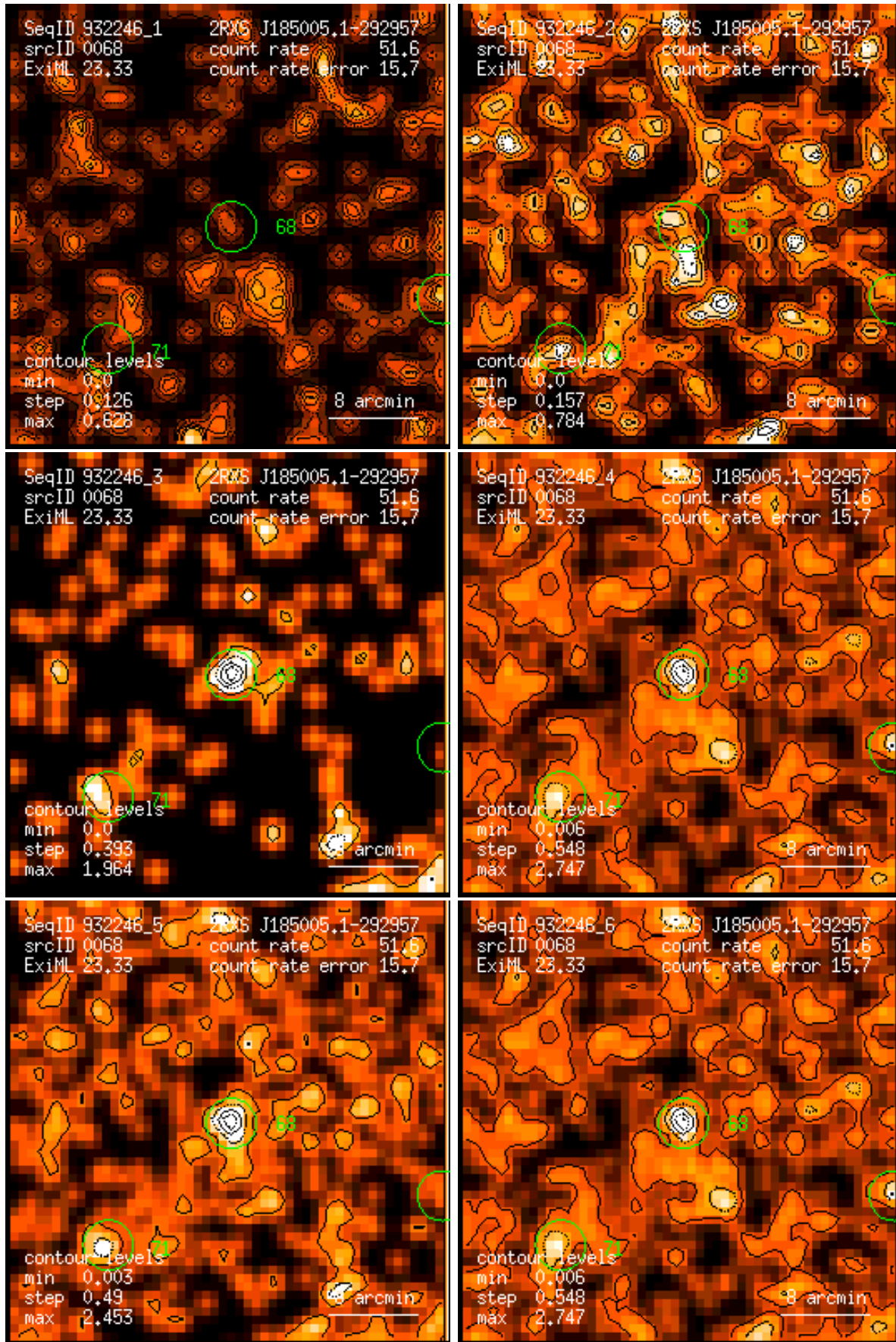
Figure 68: RASS 932246: detection 0068: band rate images, Gaussian filter: (1) PSPC channels 11 – 41, (2) 52 – 90, (3) 91 – 201, (4) 11 – 235, (5) 52 – 201, (6) 11 – 201. Broad band rates in counts/ks. Band rate contour levels in counts/ks/arcmin 2 .
