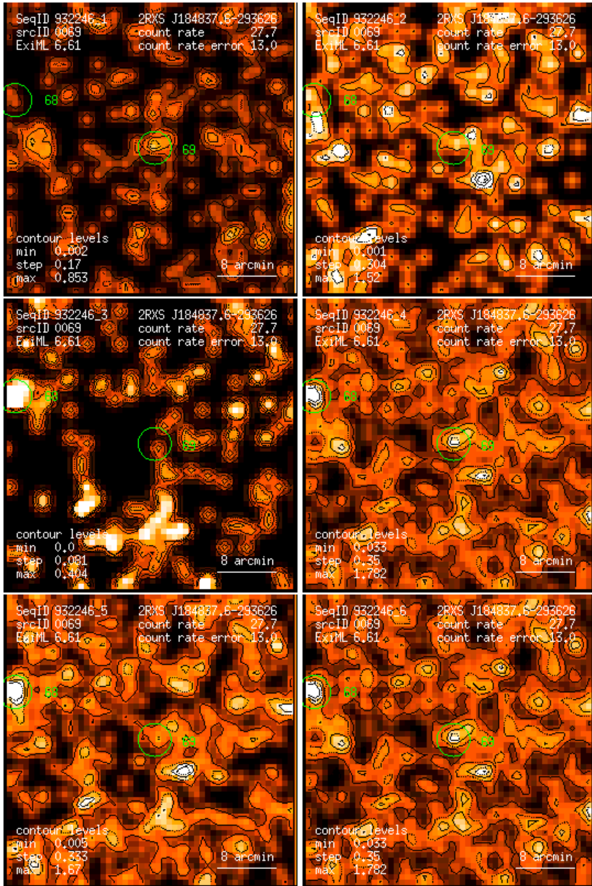
Figure 69: RASS 932246: detection 0069: band rate images, Gaussian filter: (1) PSPC channels 11 – 41, (2) 52 – 90, (3) 91 – 201, (4) 11 – 235, (5) 52 – 201, (6) 11 – 201. Broad band rates in counts/ks. Band rate contour levels in counts/ks/arcmin 2 .
