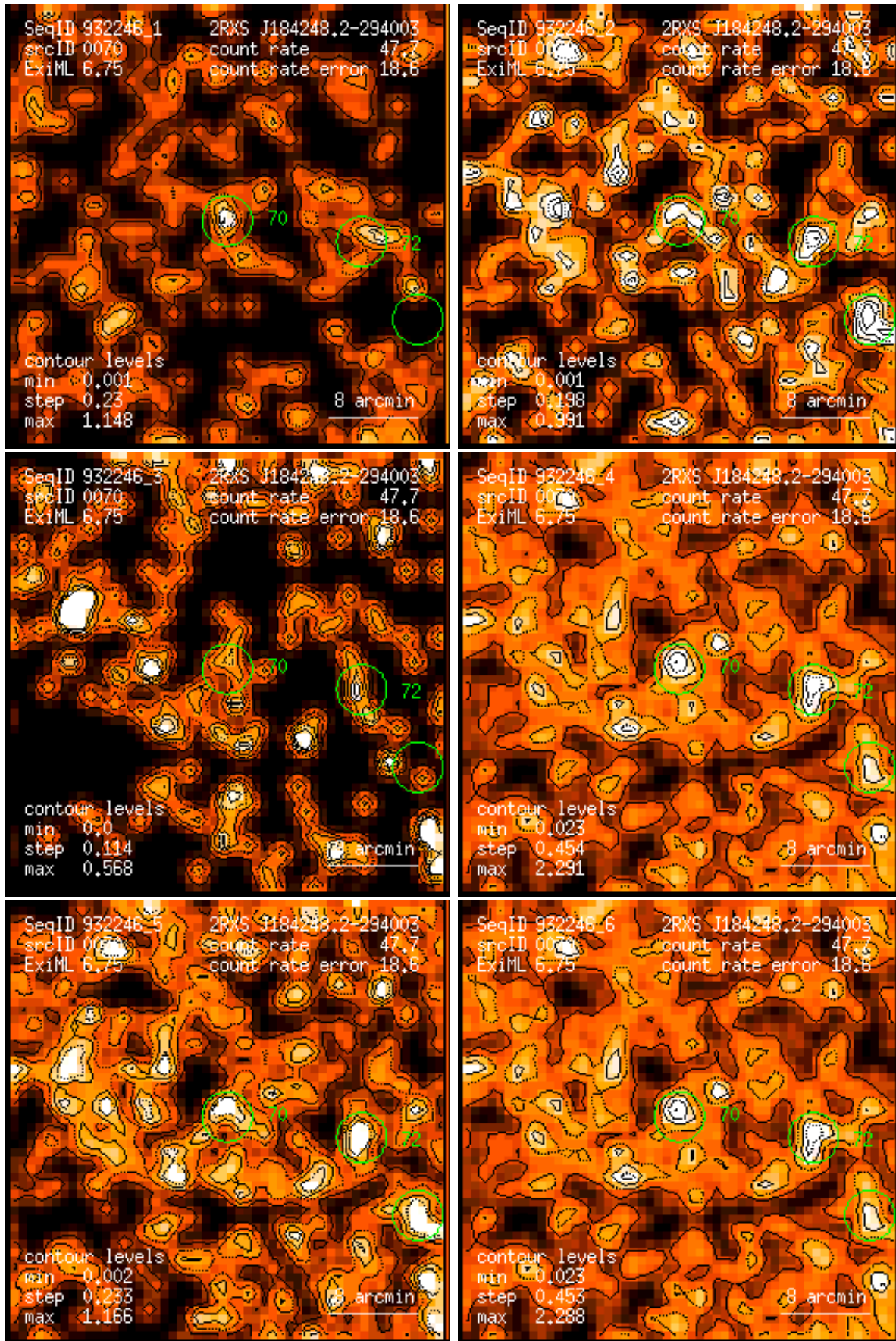
Figure 70: RASS 932246: detection 0070: band rate images, Gaussian filter: (1) PSPC channels 11 – 41, (2) 52 – 90, (3) 91 – 201, (4) 11 – 235, (5) 52 – 201, (6) 11 – 201. Broad band rates in counts/ks. Band rate contour levels in counts/ks/arcmin 2 .
