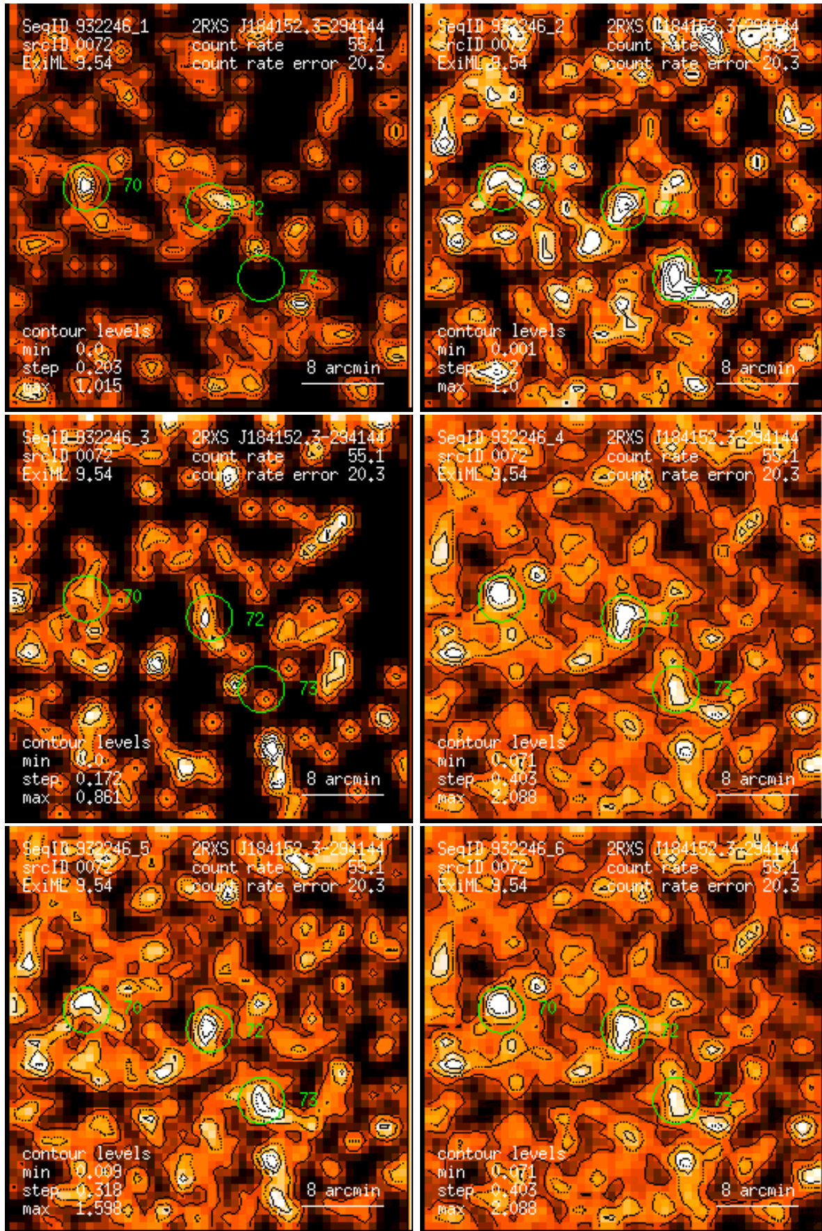
Figure 72: RASS 932246: detection 0072: band rate images, Gaussian filter: (1) PSPC channels 11 – 41, (2) 52 – 90, (3) 91 – 201, (4) 11 – 235, (5) 52 – 201, (6) 11 – 201. Broad band rates in counts/ks. Band rate contour levels in counts/ks/arcmin 2 .
