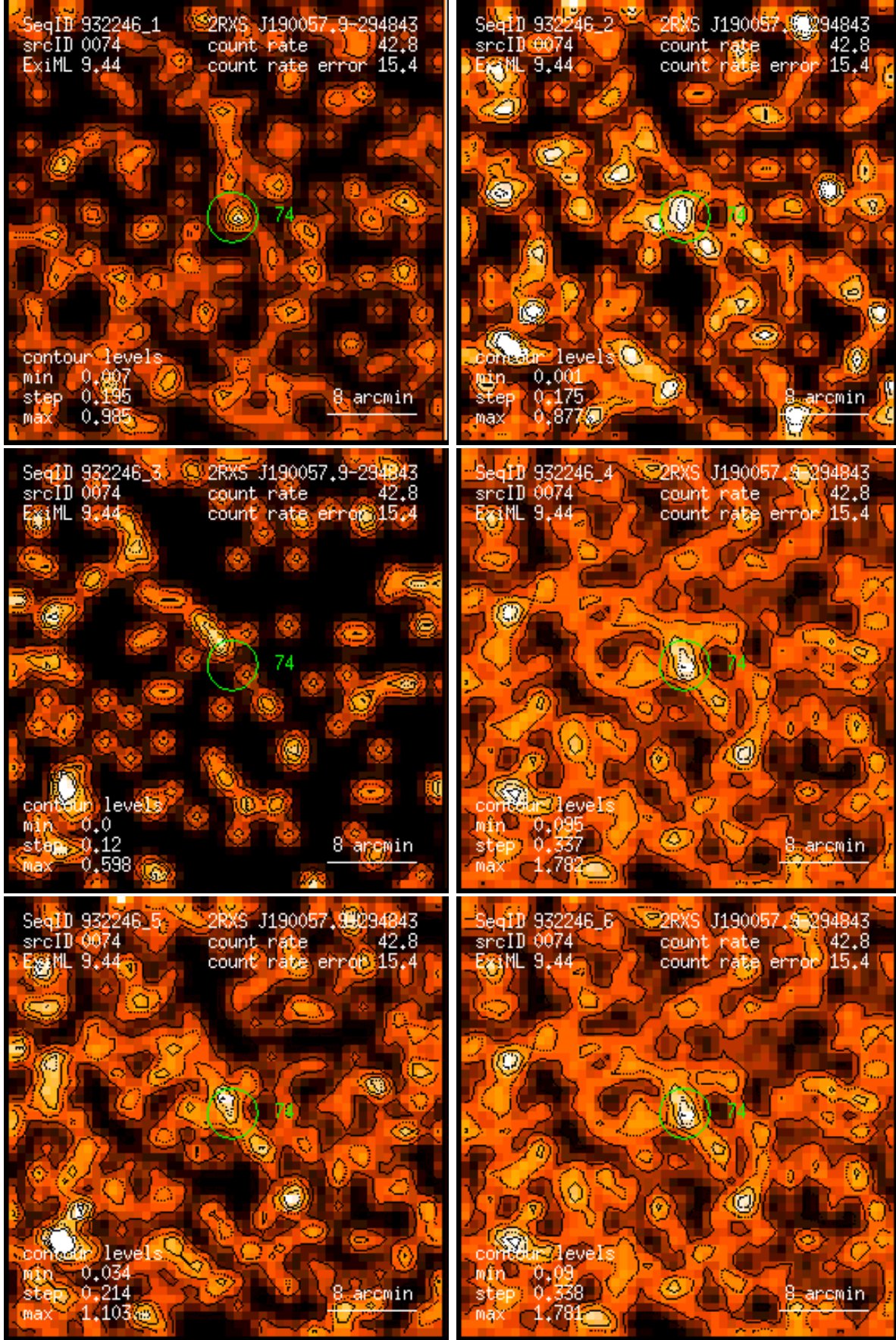
Figure 74: RASS 932246: detection 0074: band rate images, Gaussian filter: (1) PSPC channels 11 – 41, (2) 52 – 90, (3) 91 – 201, (4) 11 – 235, (5) 52 – 201, (6) 11 – 201. Broad band rates in counts/ks. Band rate contour levels in counts/ks/arcmin 2 .
