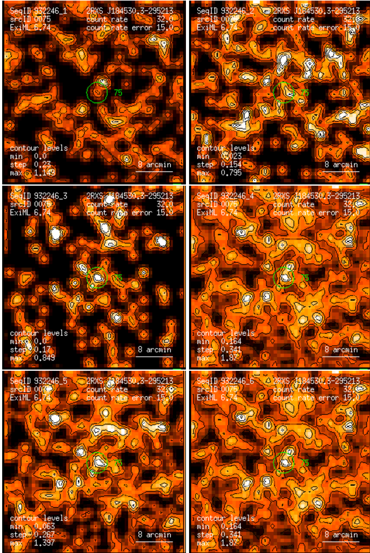
Figure 75: RASS 932246: detection 0075: band rate images, Gaussian filter: (1) PSPC channels 11 – 41, (2) 52 – 90, (3) 91 – 201, (4) 11 – 235, (5) 52 – 201, (6) 11 – 201. Broad band rates in counts/ks. Band rate contour levels in counts/ks/arcmin 2 .
