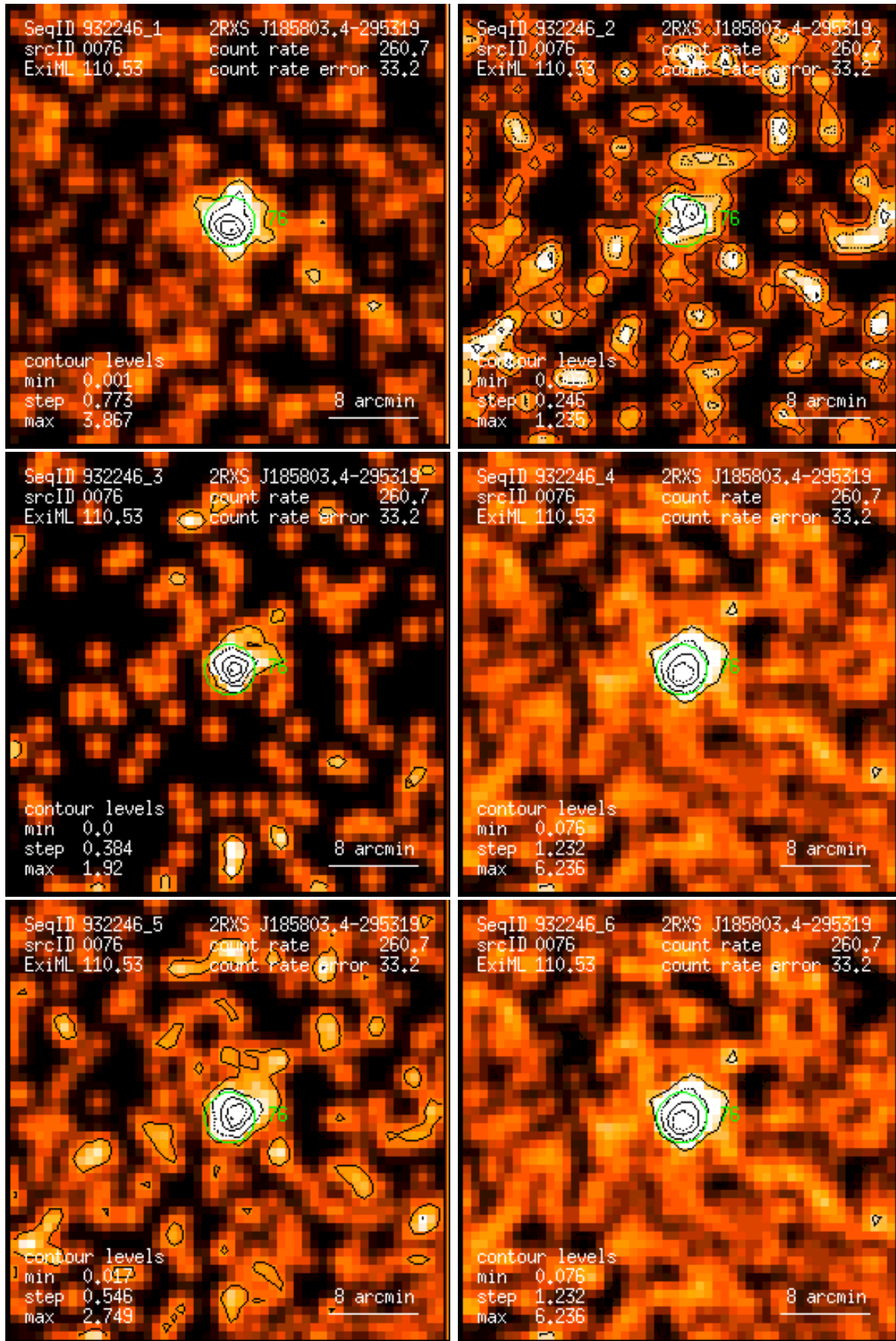
Figure 76: RASS 932246: detection 0076: band rate images, Gaussian filter: (1) PSPC channels 11 – 41, (2) 52 – 90, (3) 91 – 201, (4) 11 – 235, (5) 52 – 201, (6) 11 – 201. Broad band rates in counts/ks. Band rate contour levels in counts/ks/arcmin 2 .
