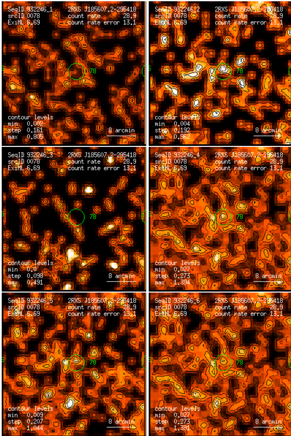
Figure 78: RASS 932246: detection 0078: band rate images, Gaussian filter: (1) PSPC channels 11 – 41, (2) 52 – 90, (3) 91 – 201, (4) 11 – 235, (5) 52 – 201, (6) 11 – 201. Broad band rates in counts/ks. Band rate contour levels in counts/ks/arcmin 2 .
